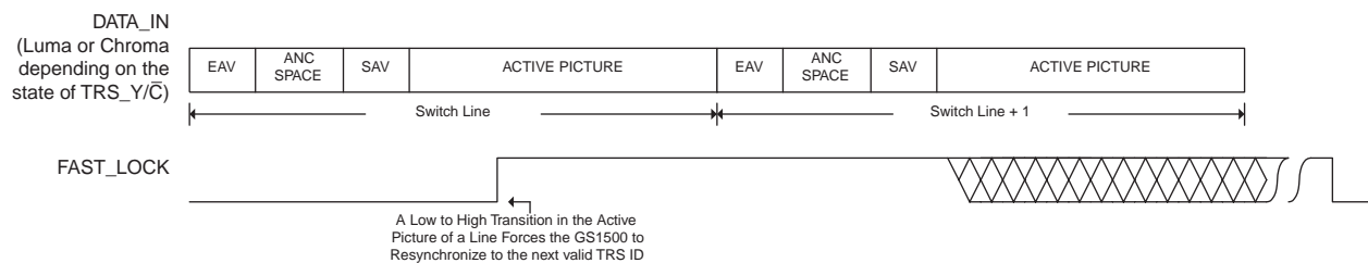
Fig. 5 FAST_LOCK Timing
