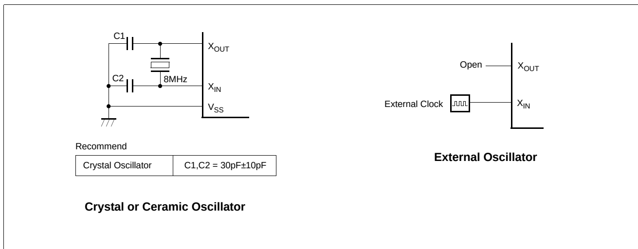
Figure 19-1 Oscillation Circuit
