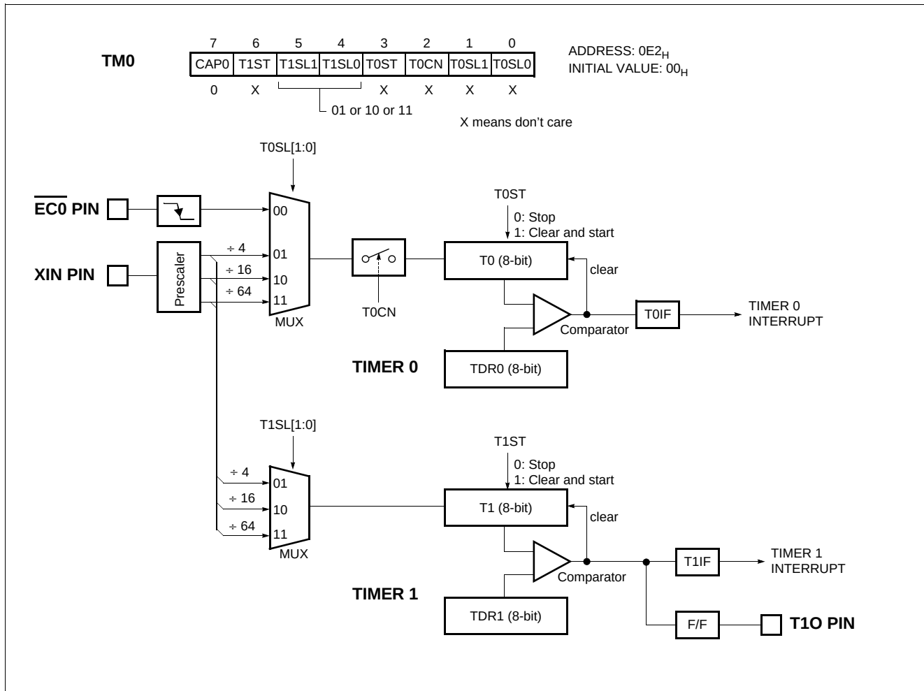
Figure 11-2 8-bit Timer/Counter 0, 1
