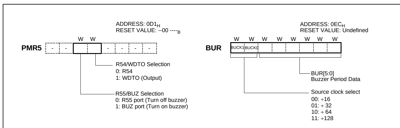
Figure 15-2 PMR5 and Buzzer Register
