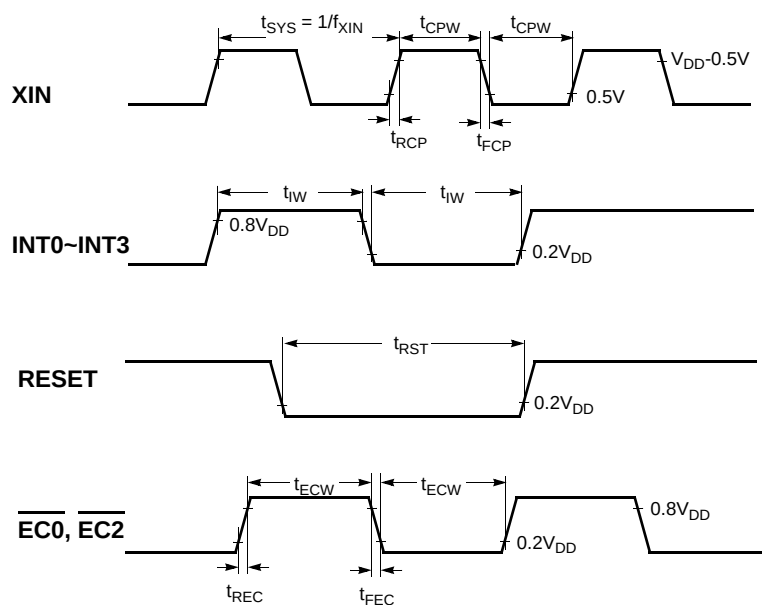
Figure 7-1 Timing Chart
