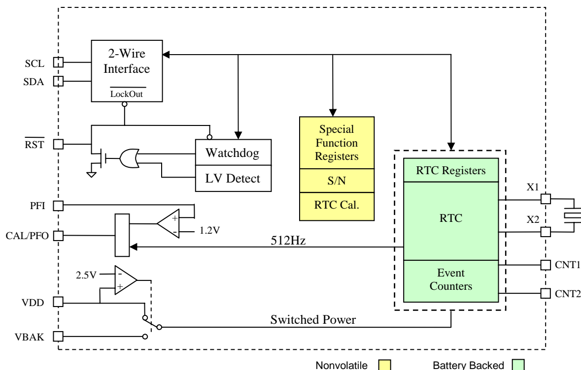
Figure 1. Block Diagram
