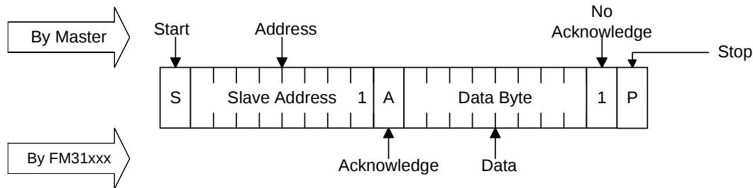
Figure 13. Current Address Memory Read
