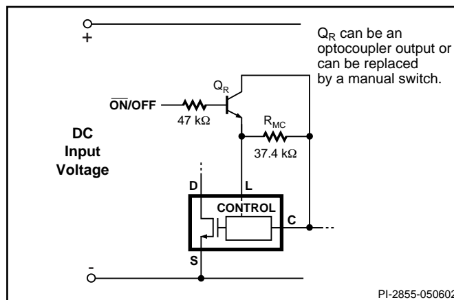
Figure 18. Active-off Remote ON/OFF. Maximum Duty Cycle will be reduced.
