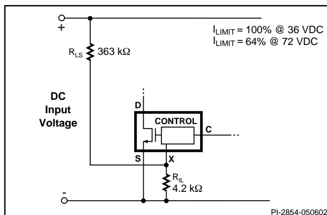
Figure 16. Current Limit Reduction with Line Voltage.
