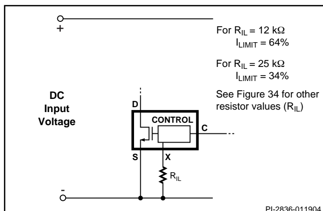
Figure 15. Externally Set Current Limit.
