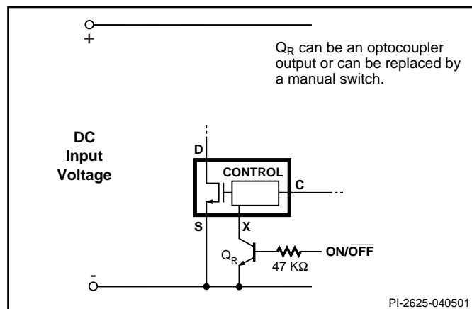
Figure 17. Active-on (Fail Safe) Remote ON/OFF.
