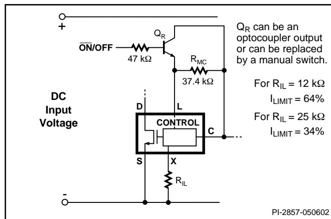
Figure 20. Active-off Remote ON/OFF with Externally Set Current Limit.
