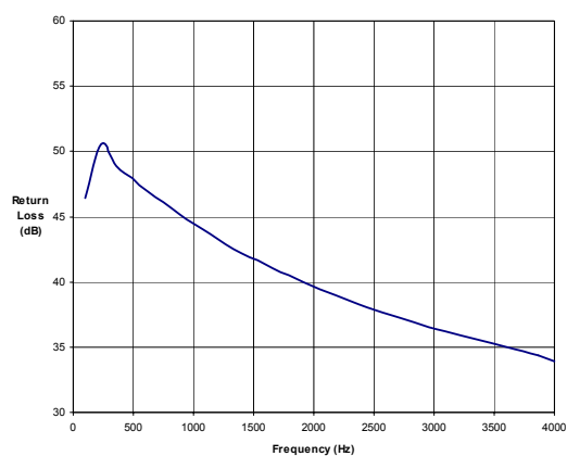
Figure 13. Return Loss
