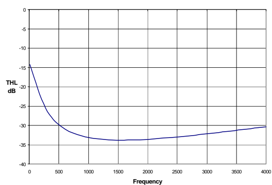
Figure 12. Trans-Hybrid Loss
