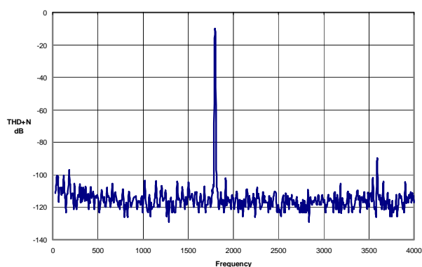
Figure 11. Transmit THD on Tip and Ring
