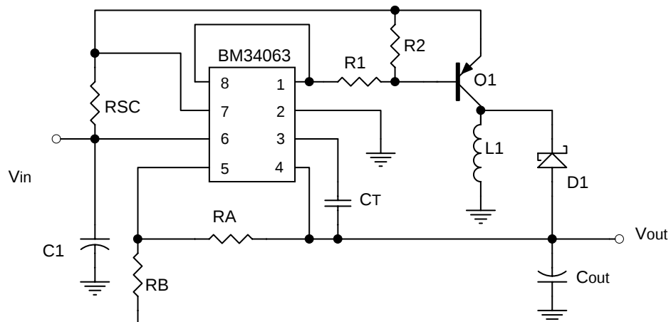
Fig.7 Voltage Inverting Converter With External PNP Saturation Switch
