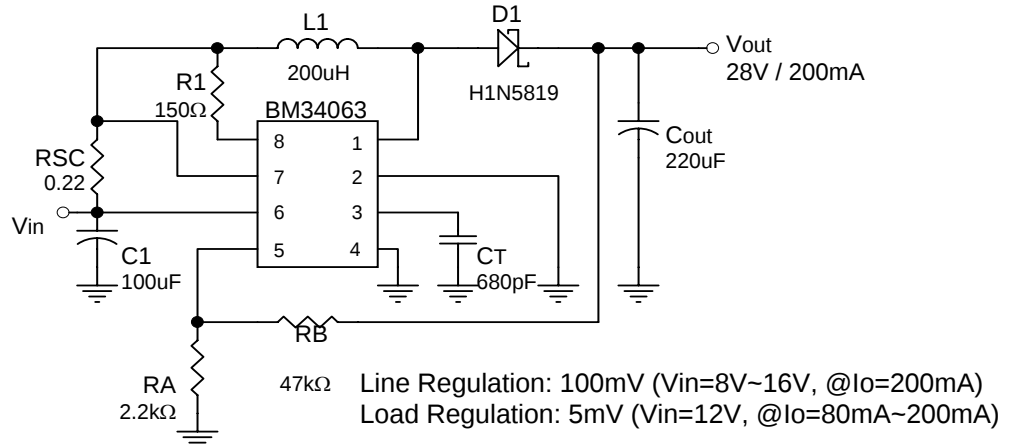
Fig.2 Step-Up Converter
