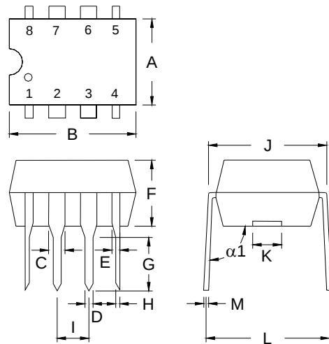
8-Lead DIP-8 Plastic Package
