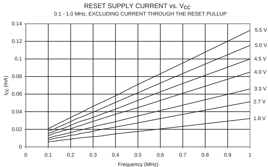
Figure 138. Reset Supply Current vs. V_{CC} (0.1 - 1.0 MHz, Excluding Current Through The Reset Pull-up)
