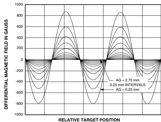
Magnetic signal
