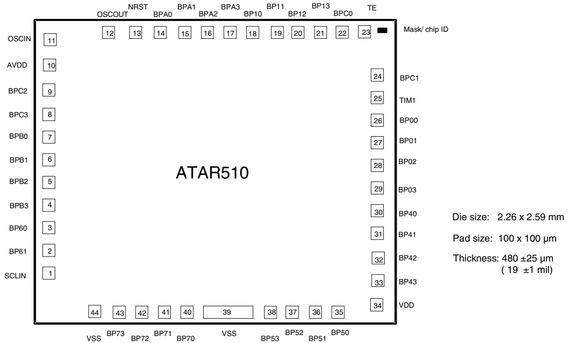
Figure 8-1. Pad Assignments
