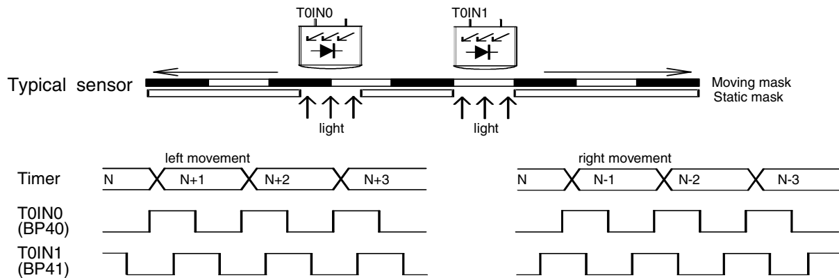
Figure 3-23. Position Measurement Mode
