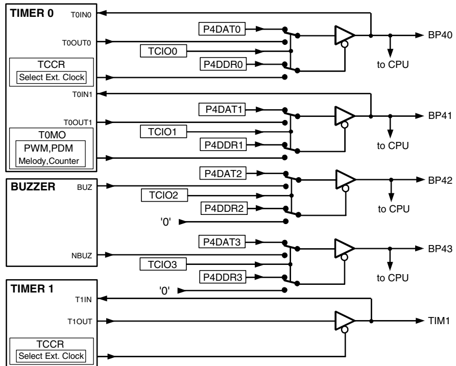
Figure 3-12. Timer/Counter and Buzzer External Interface
