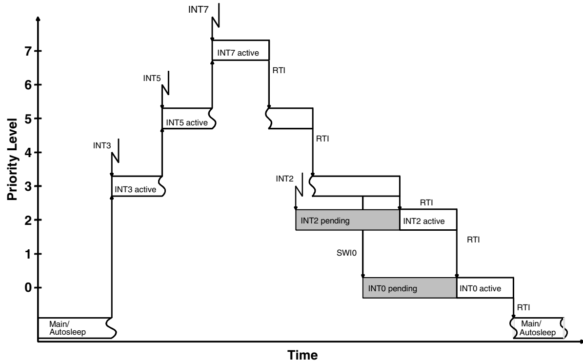
Figure 2-6. Interrupt Handling
