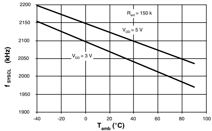
Figure 7-5. f_{\text{SYSCL}} = f(T_{\text{amb}}) ; External RC
