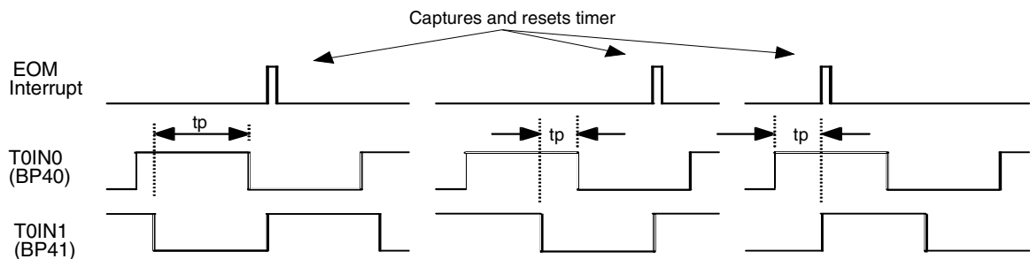
Figure 3-22. Phase Measurement
