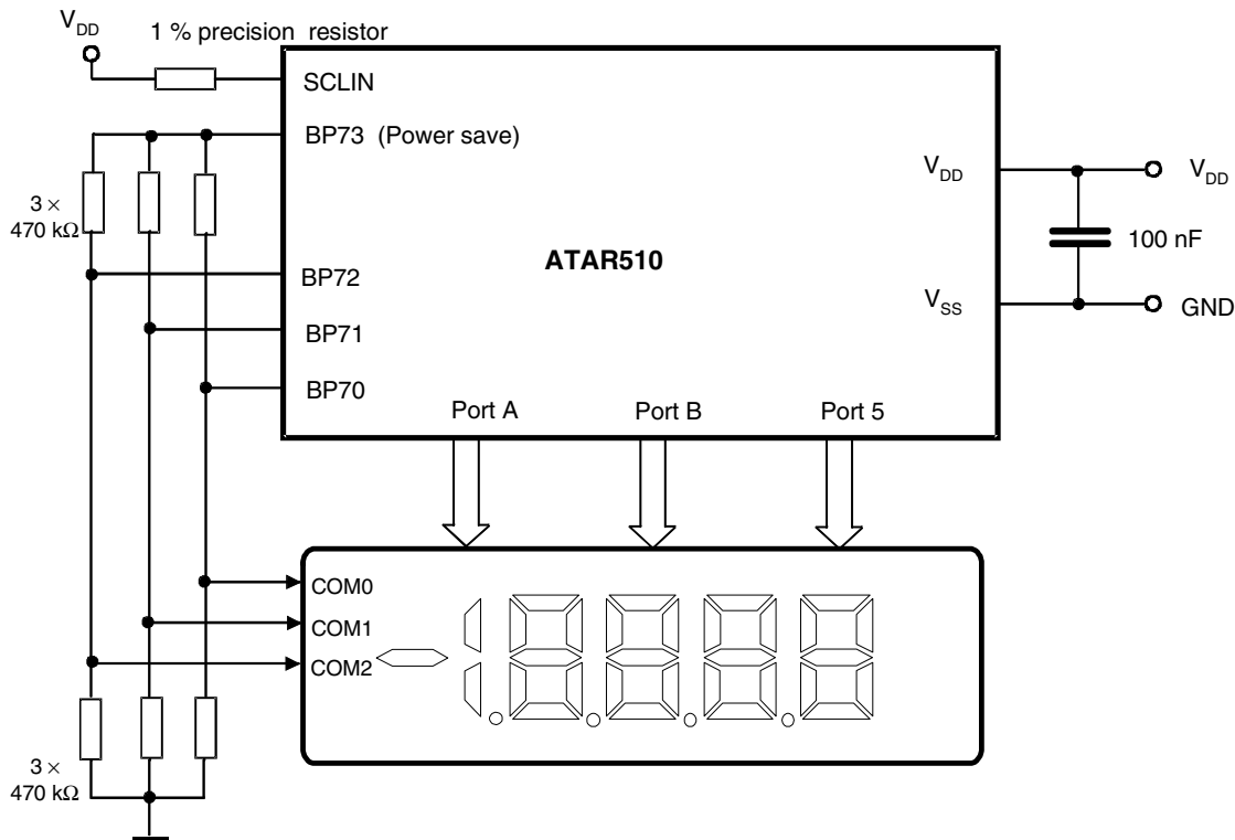
Figure 9-2. Driving a LCD Panel with 1/3 Duty
