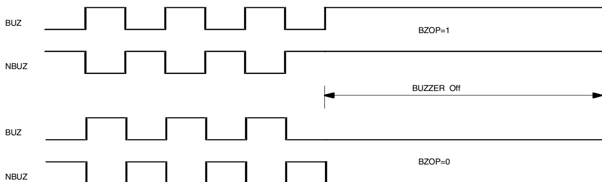
Figure 3-28. Buzzer Waveform
