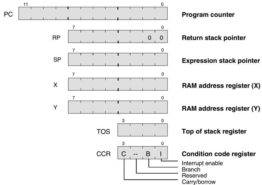
Figure 2-4. Programming Model
