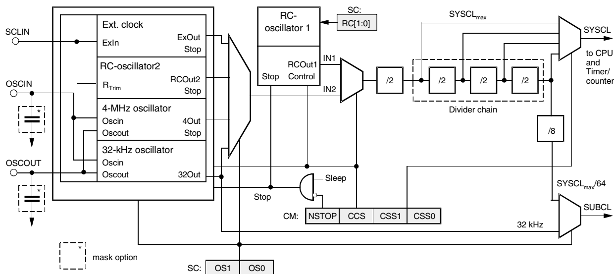
Figure 2-8. Clock Module
