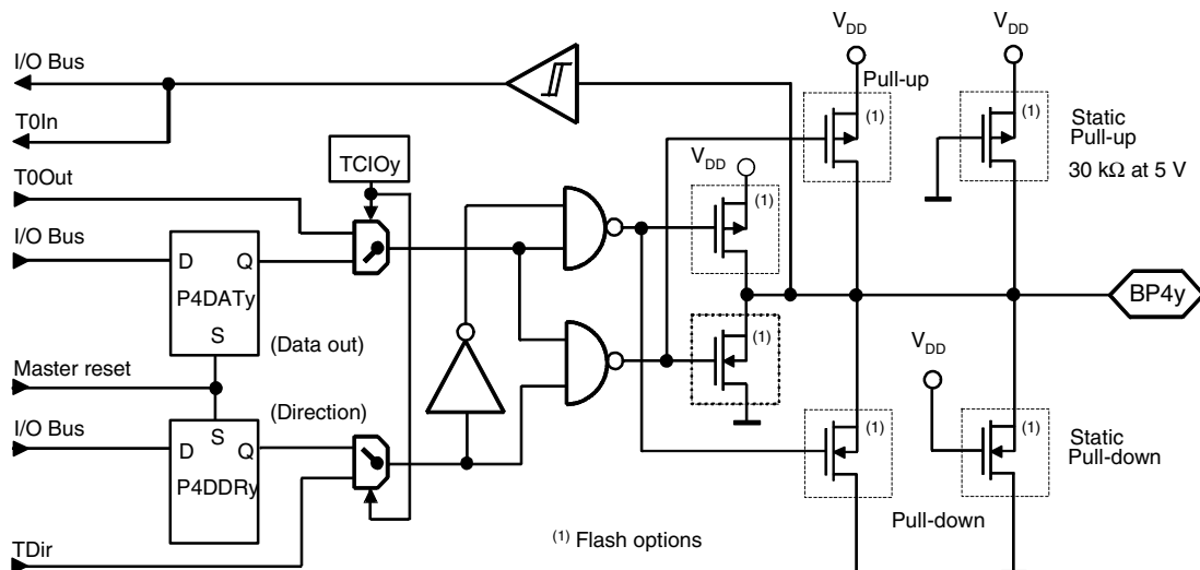
Figure 3-7. Bi-directional Port 4
