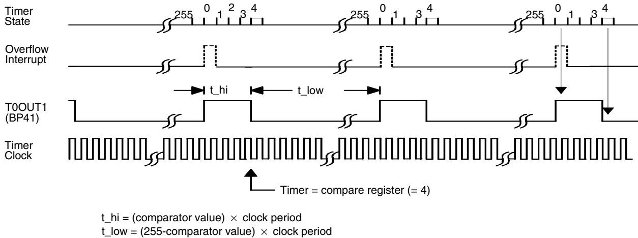
Figure 3-18. Timer 0 Pulse Width Modulation
