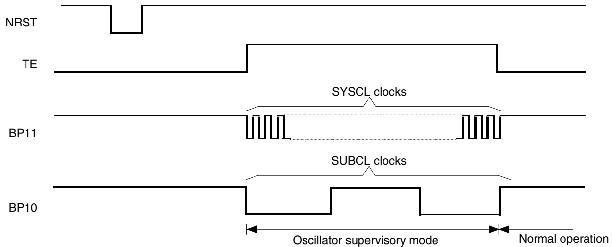
Figure 2-14. Clock Monitoring
