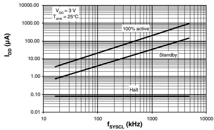
Figure 7-3. I_{DD} = f(f_{SYSC\_L}), V_{DD} = 3\text{ V}
