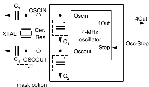
Figure 2-12. System Clock Oscillator
