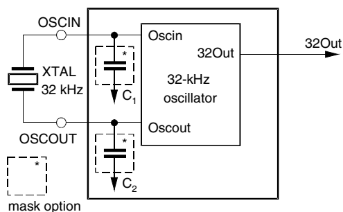
Figure 2-13. 32-kHz Crystal Oscillator
