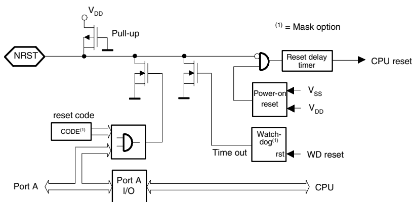
Figure 2-7. Reset Configuration
