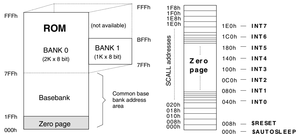
Figure 2-2. ROM Map
