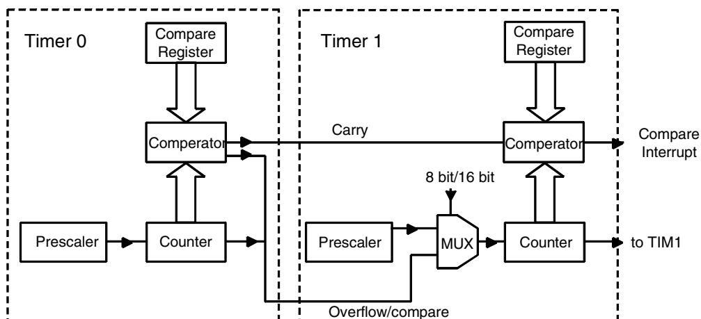
Figure 3-13. 16-bit Mode
