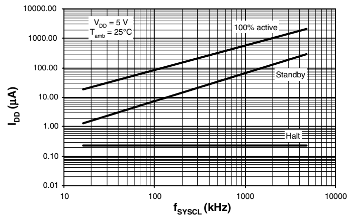
Figure 7-4. I_{DD} = f(f_{SYSC\_L}), V_{DD} = 5\text{ V}
