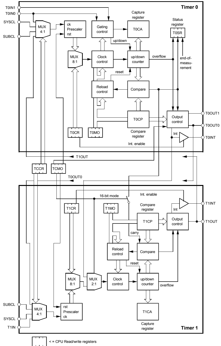
Figure 3-11. Timer/Counter Module
