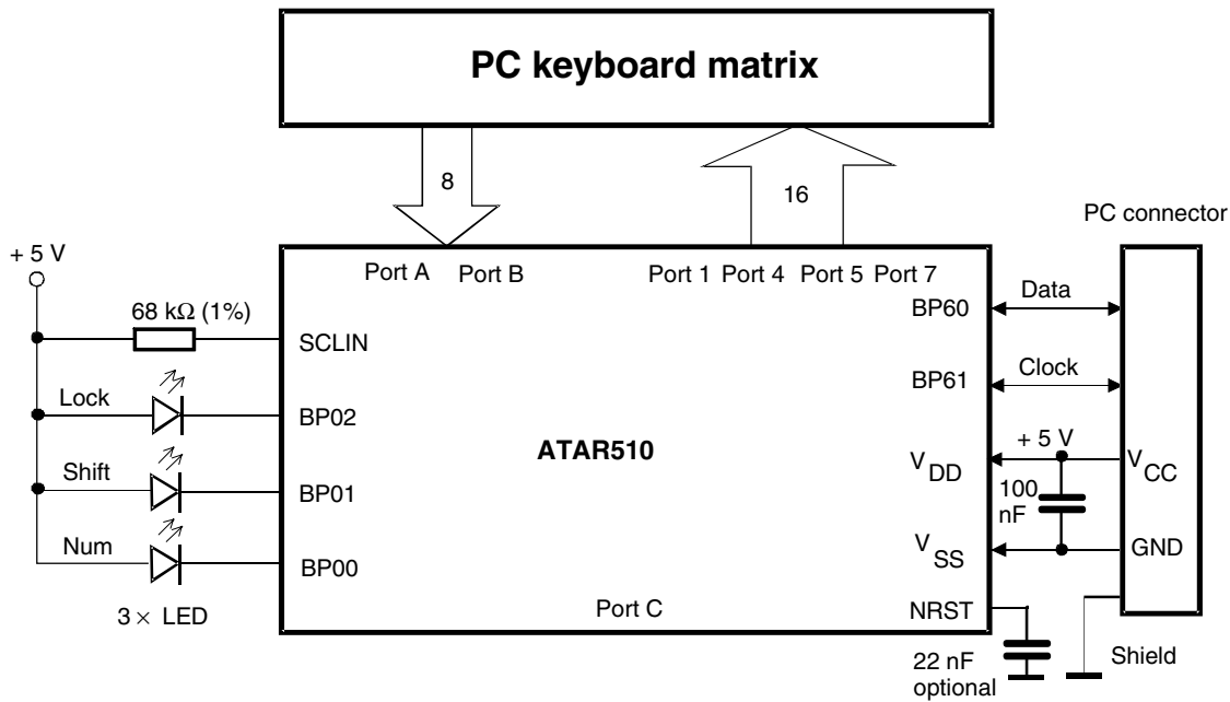
Figure 9-1. ATAR510 as Keyboard Controller
