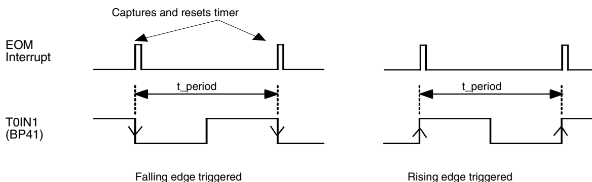
Figure 3-20. Period Measurement
