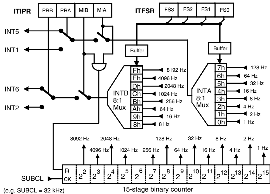
Figure 3-9. Interval Timers/Prescaler
