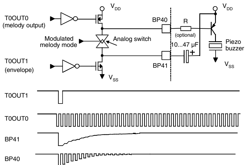
Figure 3-17. Modulated Melody Output Circuit
