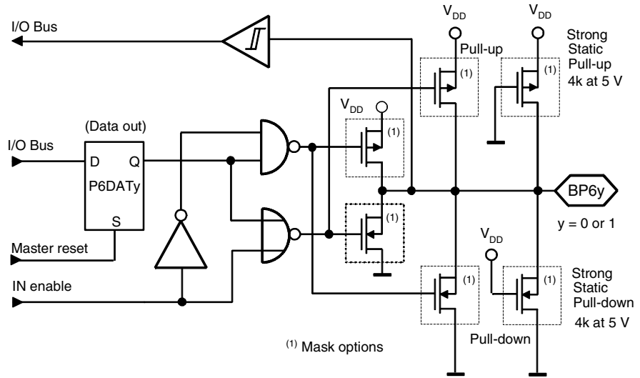
Figure 3-5. Bi-directional Port 6
