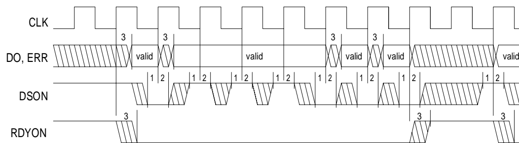
Figure 11: Data Output
