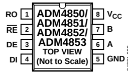
Figure 2. ADM4850–ADM4853 Pin Configuration
