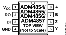
Figure 3. ADM4854–ADM4857 Pin Configuration
