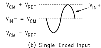
FIGURE 2. Expected Input Signal Range
