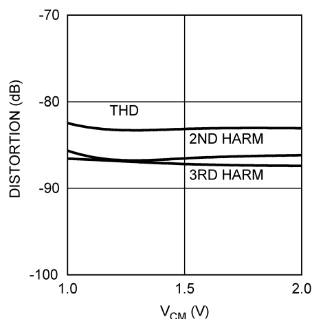
Distortion vs. V_{CM}
