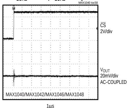
MAJOR CARRY TRANSITION R LOAD = 10kΩ, C LOAD = 100pF
