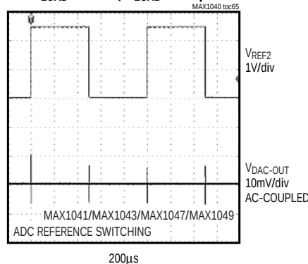
ADC REFERENCE FEEDTHROUGH R LOAD = 10kΩ, C LOAD = 100pF
