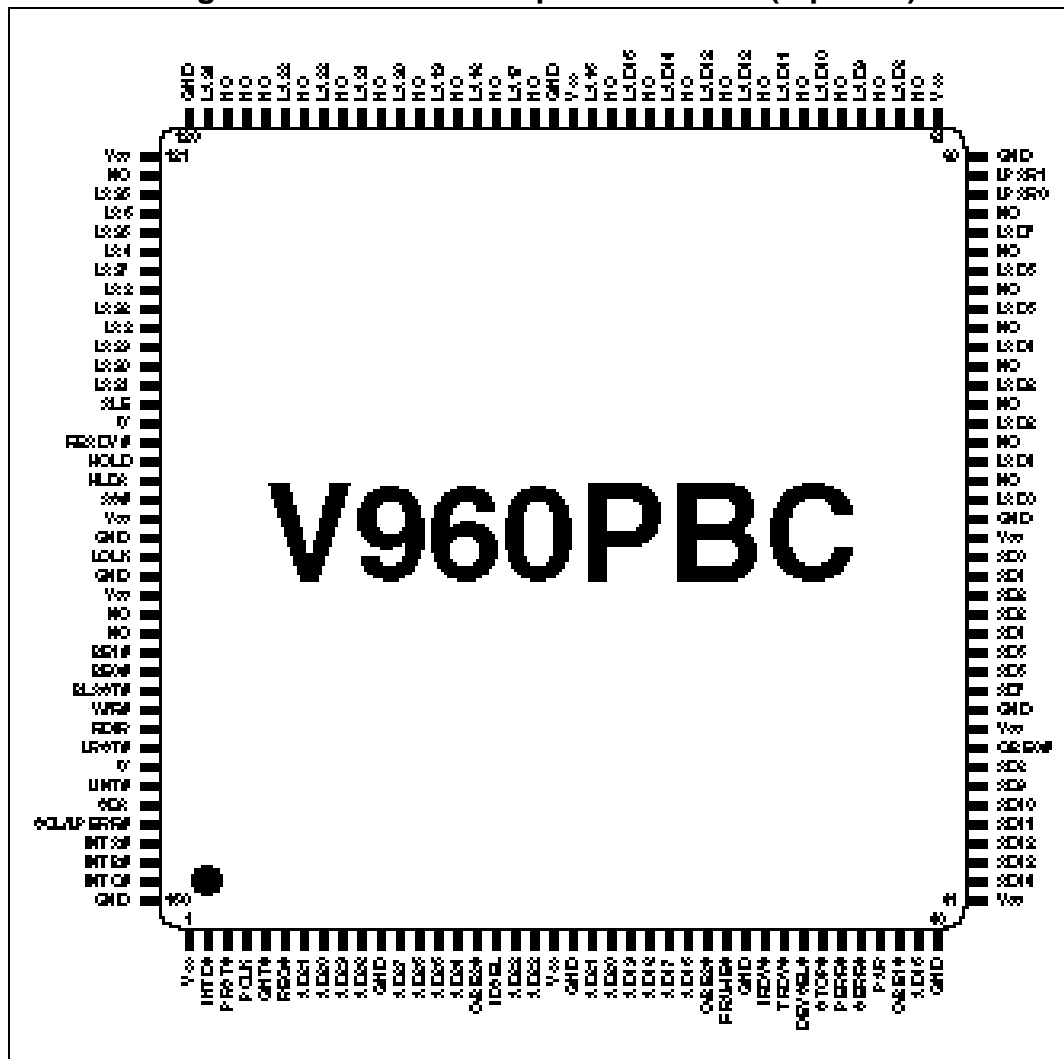
Figure 1: Pinout for 160-pin ElAJ PQFP (top view)
