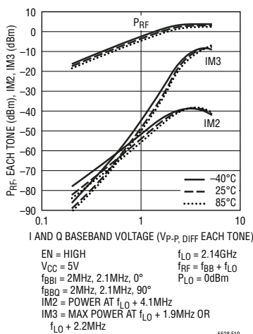
Figure 19: RF Two-Tone Power, IM2 and IM3 at 2140MHz vs Baseband Voltage
