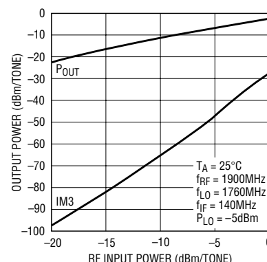
IF Output Power and IM3 vs RF Input Power (Two Input Tones)
