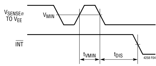
Figure 4. DC Disconnect Timing
