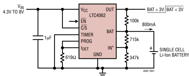
800mA Single Cell Li-Ion Battery Charger (C/10 Termination)
