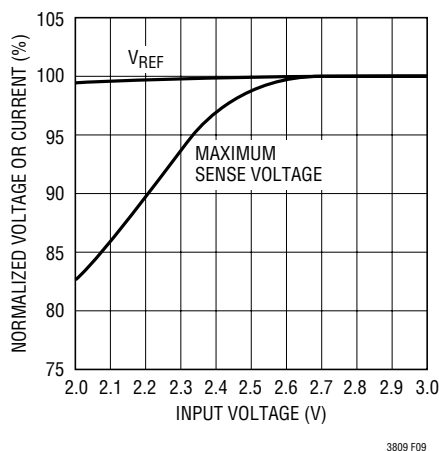
Figure 9. Line Regulation of V_{REF} and Maximum Sense Voltage
