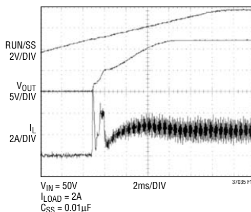
Figure 17. LTC3703-5 Startup Operation
