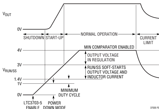
Figure 3. Soft-Start Operation in Start Up and Current Limit
