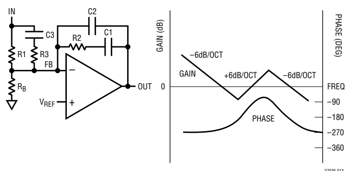
Figure 13. Type 3 Schematic and Transfer Function
