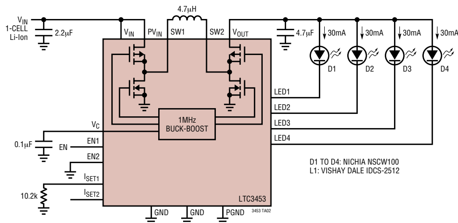
High Efficiency 4 White LED Driver
