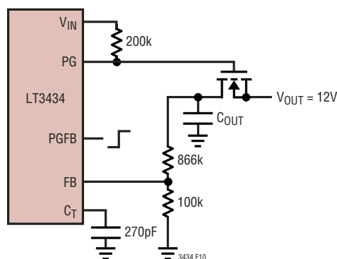
V_{OUT} Disconnect 3.3V Logic Signal with 100μs Delay
