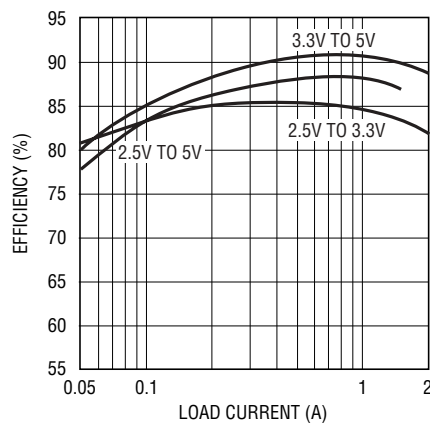
Converter Efficiency
