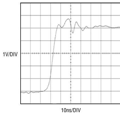
SWA, SWB Rise Time, I = 2A
