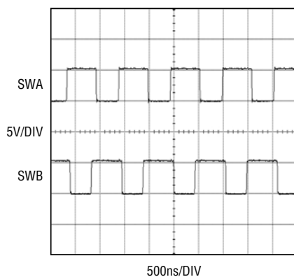
SWA, SWB Switching Waveforms
