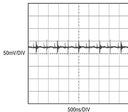
Output Voltage Ripple with 22μF Ceramic Capacitor
