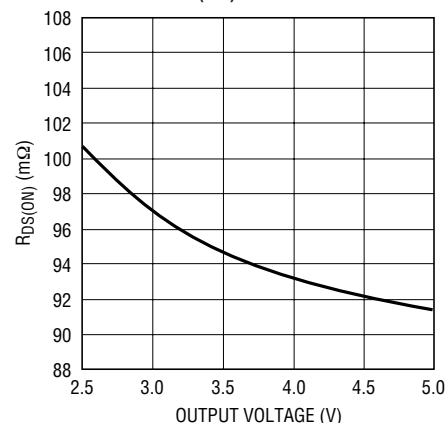
Switch R_{DS(ON)} vs V_{OUT}
