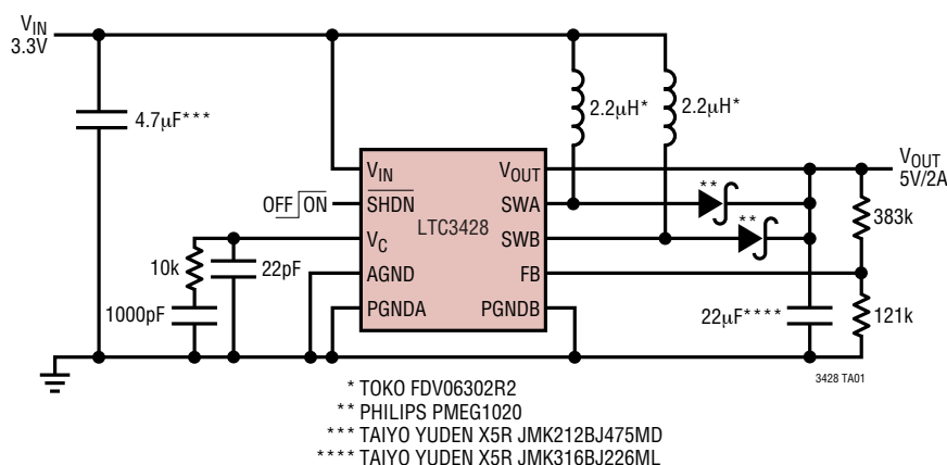
3.3V to 5V at 2A Converter
