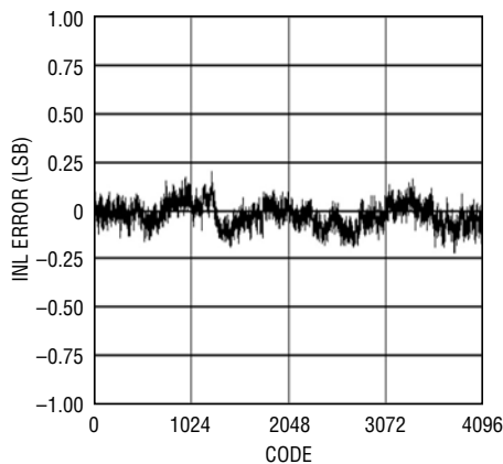
LTC2291: Typical INL, 2V Range, 25Mps
