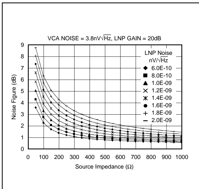
FIGURE 6. Noise Figure for Active Termination.
