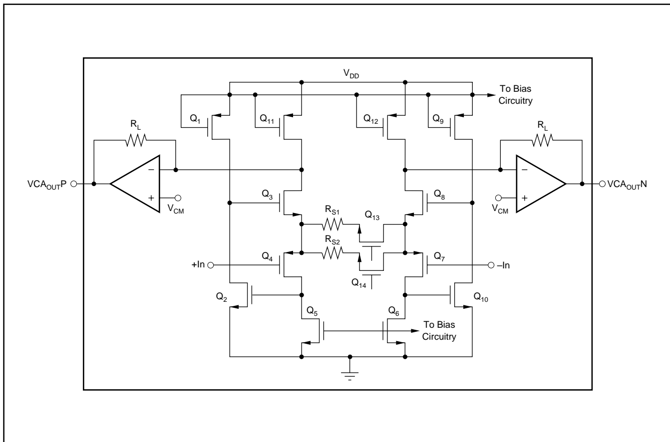
FIGURE 15. Simplified Block Diagram of the PGA Section Within the VCA2616.
