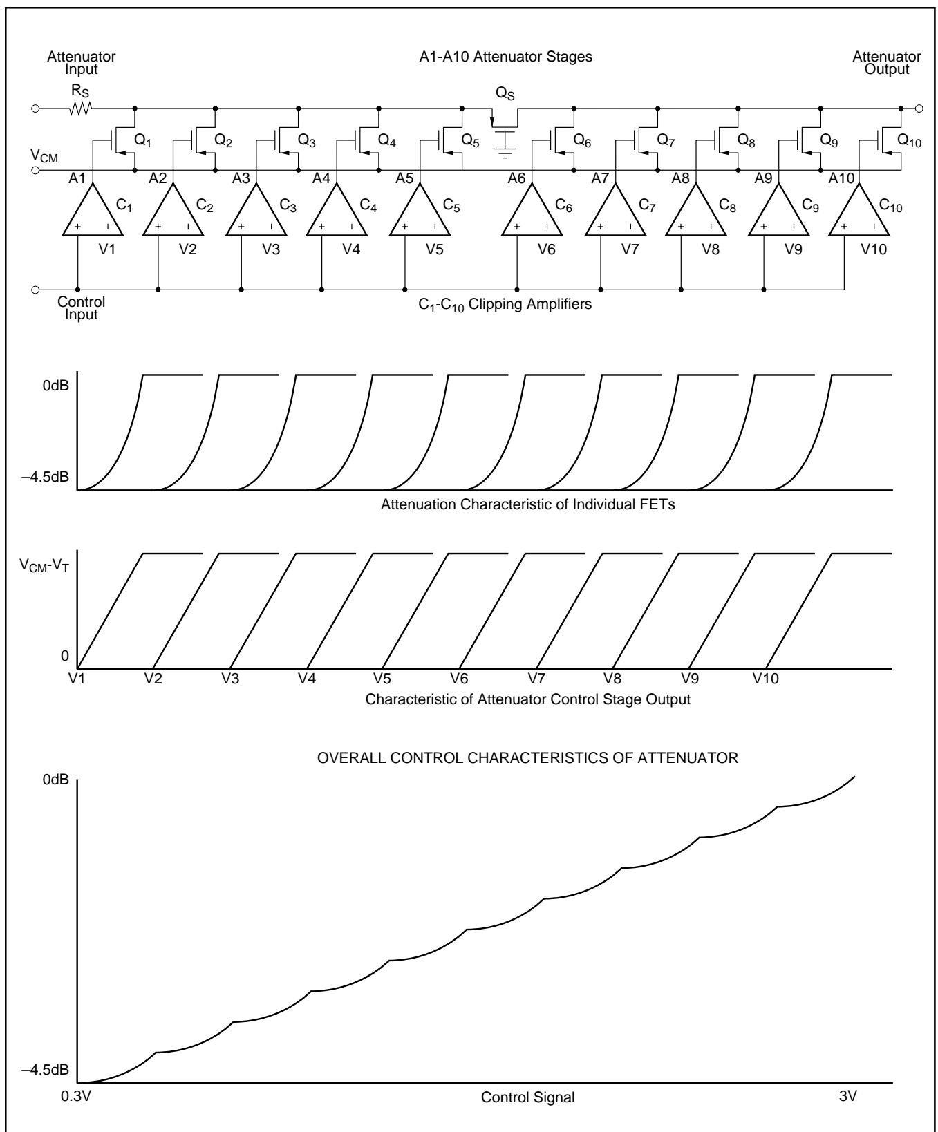
FIGURE 13. Piecewise Approximation to Logarithmic Control Characteristics.
