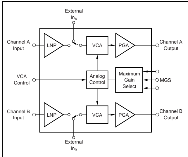
FIGURE 1. Simplified Block Diagram of the VCA2616.
