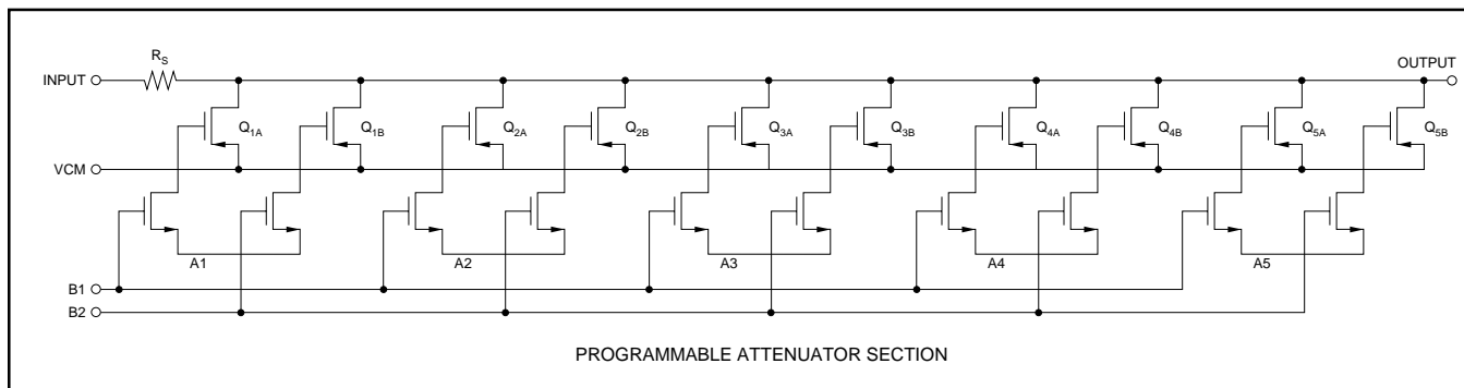
FIGURE 12. Programmable Attenuator Section.
