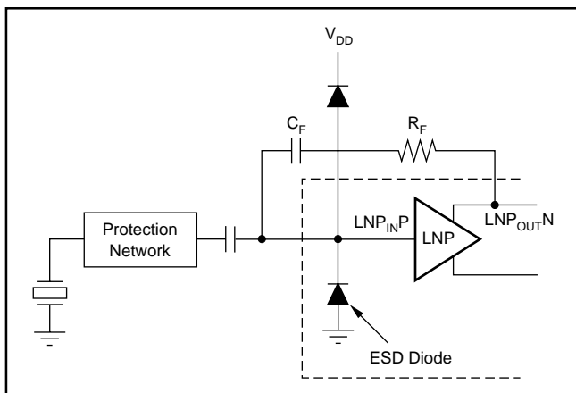
FIGURE 14. VCA2616 Diode Bridge Protection Circuit.
