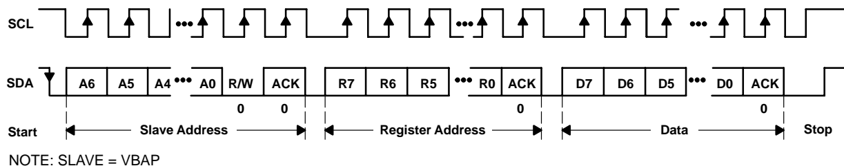
Figure 1. I²C Bus Write to VBAP
