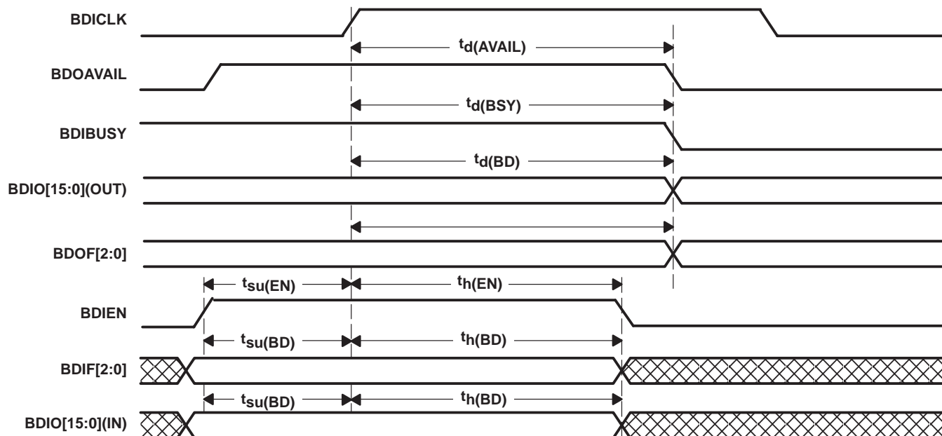
Figure 9–1. Synchronous Mode
