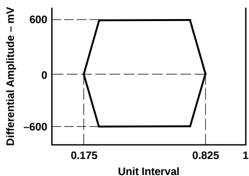
Figure 4-2. Transmit Template
