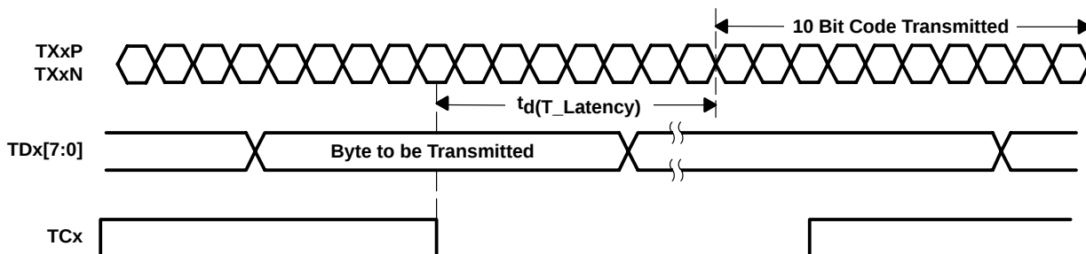
Figure 3–2. Transmitter Latency
