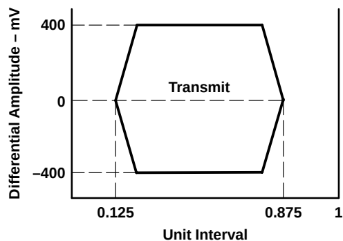
Figure 11. Transmit Template
