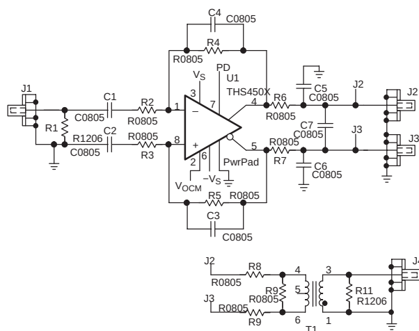
Simplified Schematic of the Evaluation Board. Power Supply Decoupling, VCM, and Power Down Circuitry Not Shown
