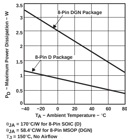
Figure 117. Maximum Power Dissipation vs Ambient Temperature
