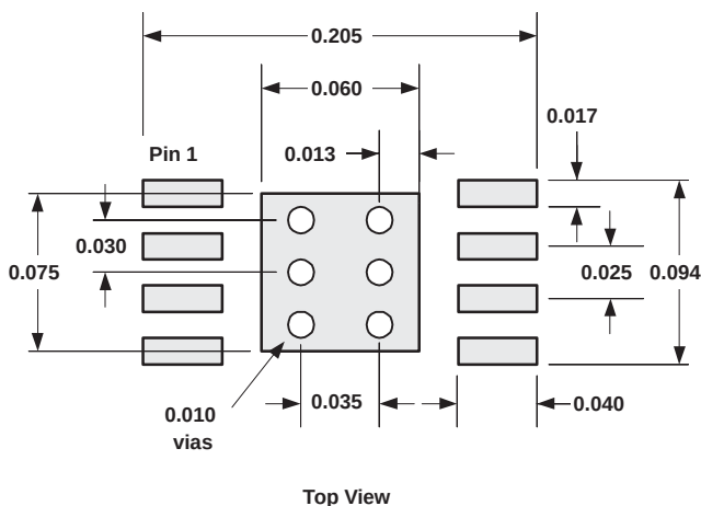
Figure 116. PowerPAD PCB Etch and Via Pattern
