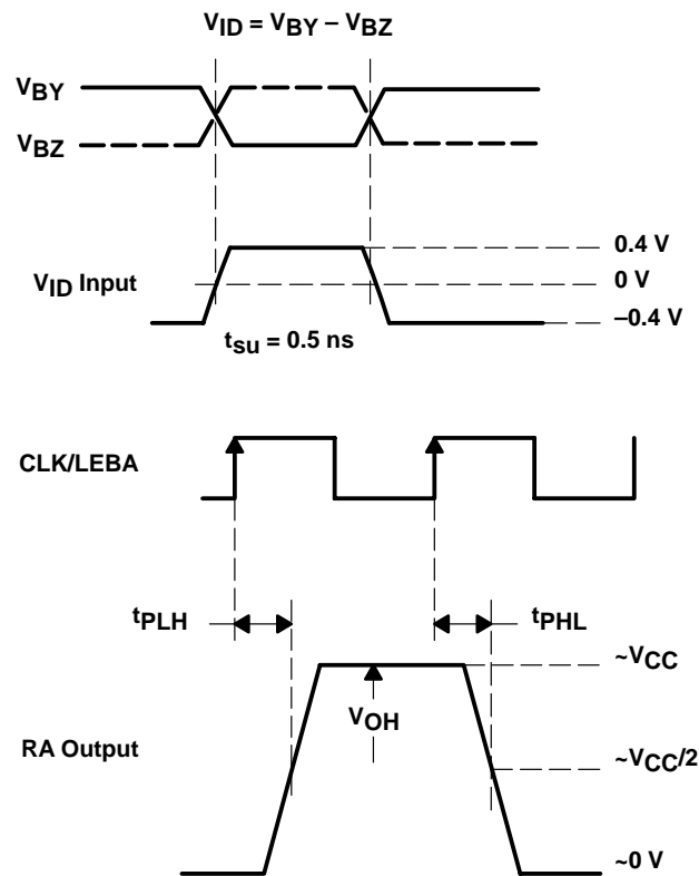
Figure 23. B-to-A Flip-Flop Mode Timing Circuit
