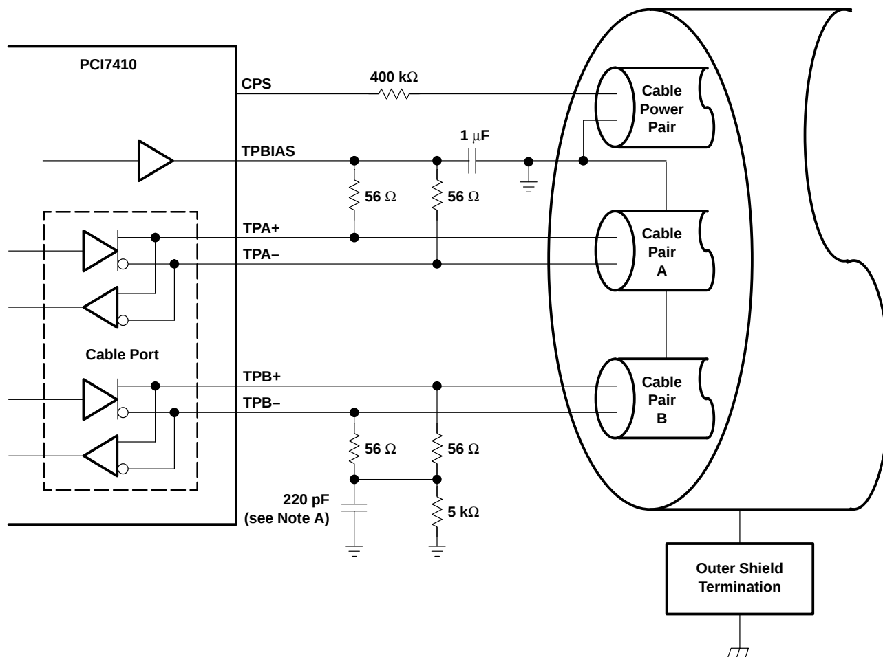
Figure 3–19. TP Cable Connections
