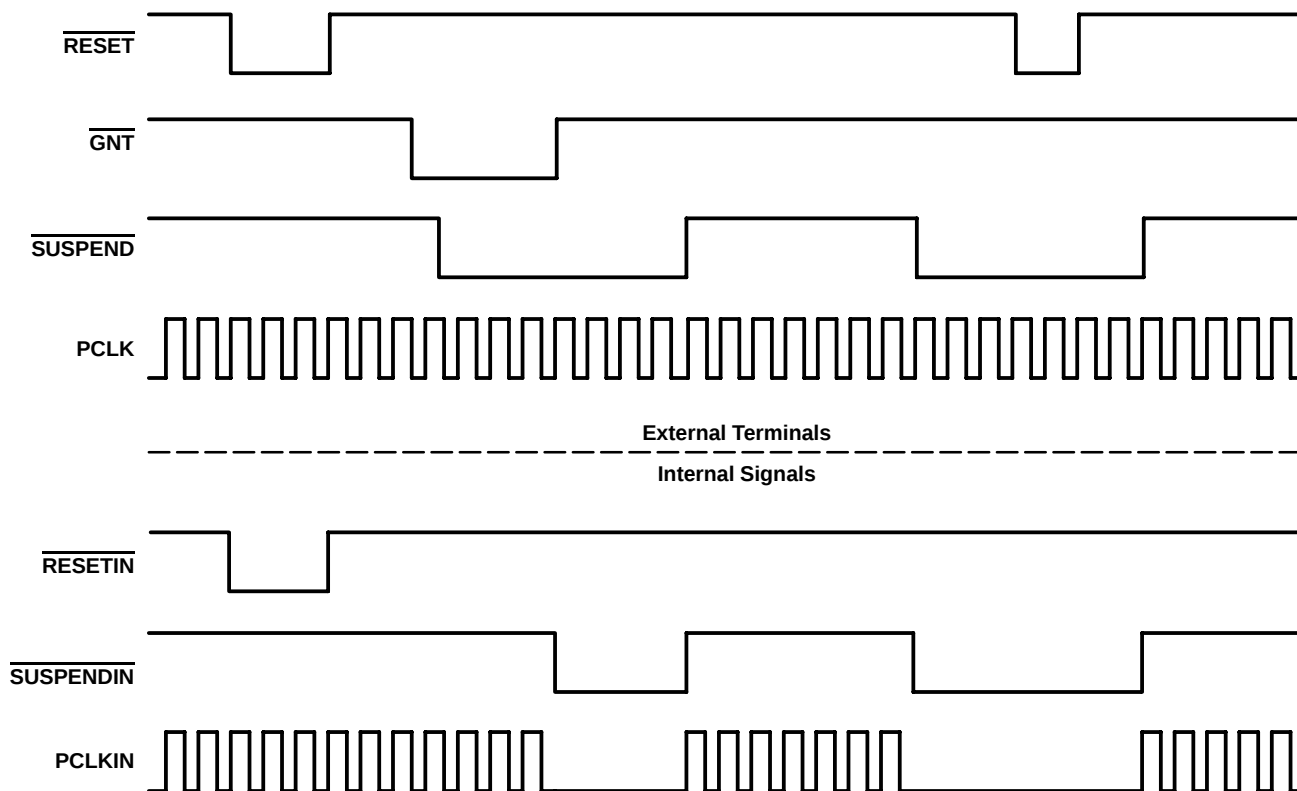
Figure 3–16. Signal Diagram of Suspend Function
