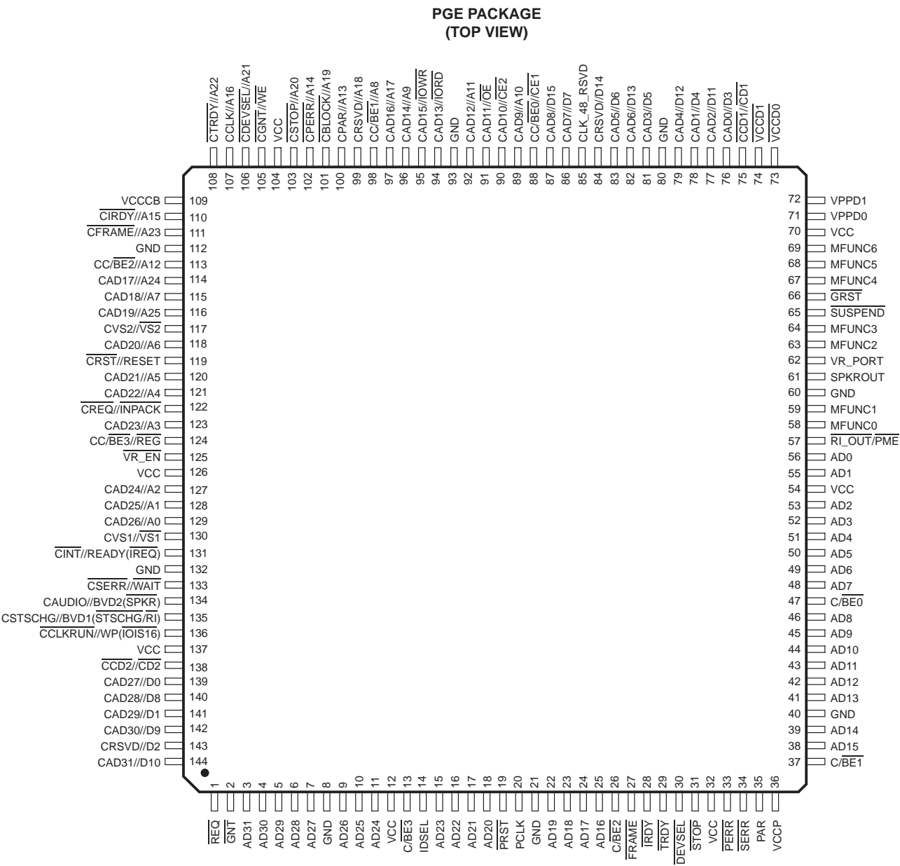
Figure 2-2. PCI1510 PGE-Package Terminal Diagram
