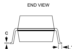
Package Dimensions for SOT23-6.
