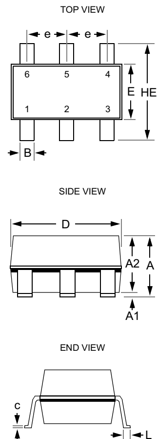
Package Dimensions for SC70-6.
