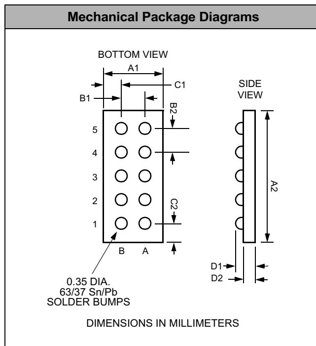
Package Dimensions for PACDN1408C 10-bump Chip Scale Package
