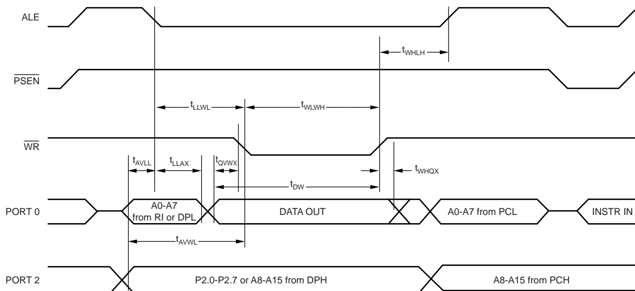
FIGURE C. External Data Memory Write Cycle
