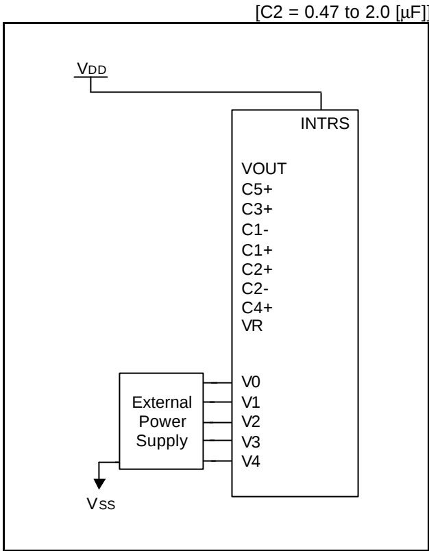
Figure 26. When Not Using any Internal LCD Power Supply Circuits (V/C: OFF, V/R: OFF, V/F: OFF)
