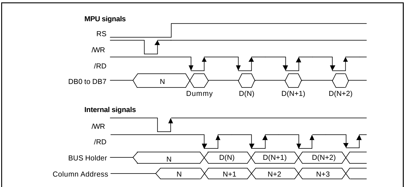
Figure 8. Read Timing
