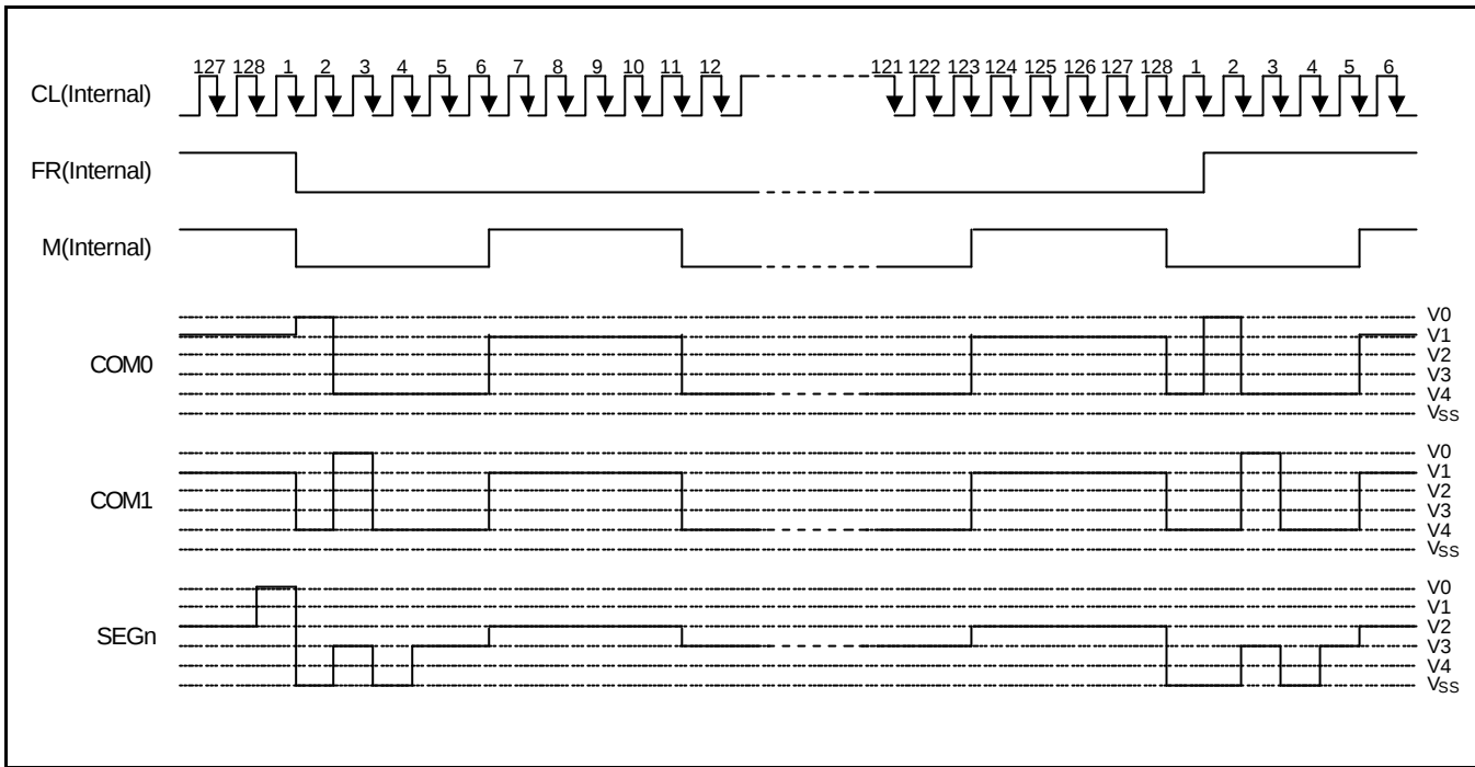
Figure 12. N-Line Inversion Driving Waveform (N = 5, Duty Ratio = 1/128)
