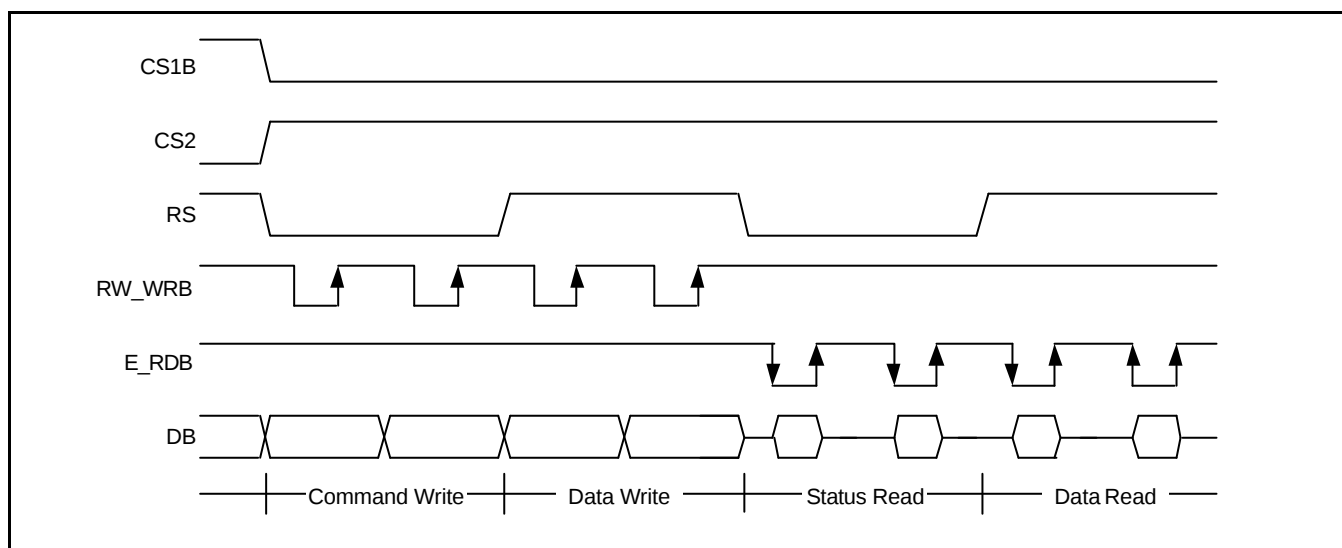
Figure 2-2. 8080-Series MPU Interface Protocol (PS="H", C68="L")
