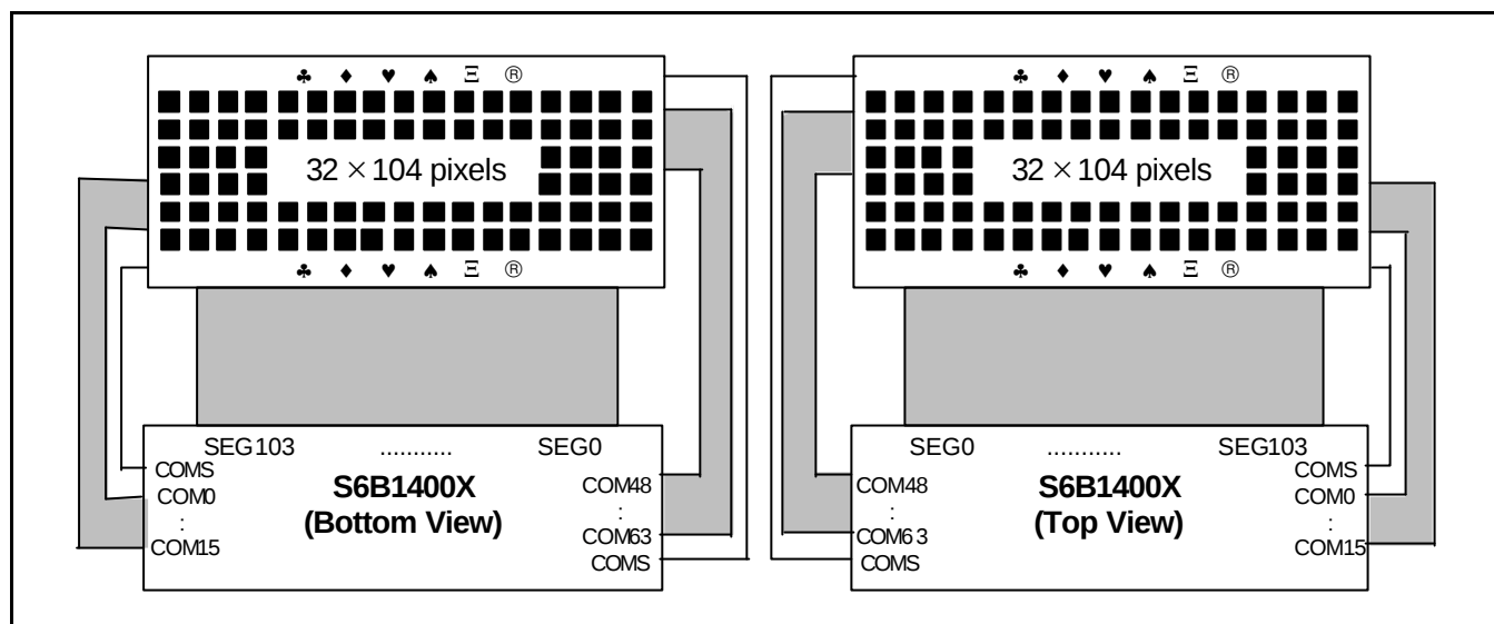
Figure 45. SHL = 1, ADC = 1
