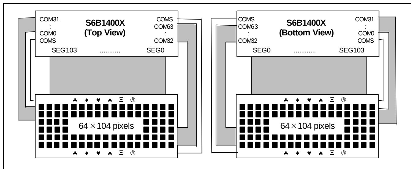
Figure 35. SHL = 0, ADC = 1
