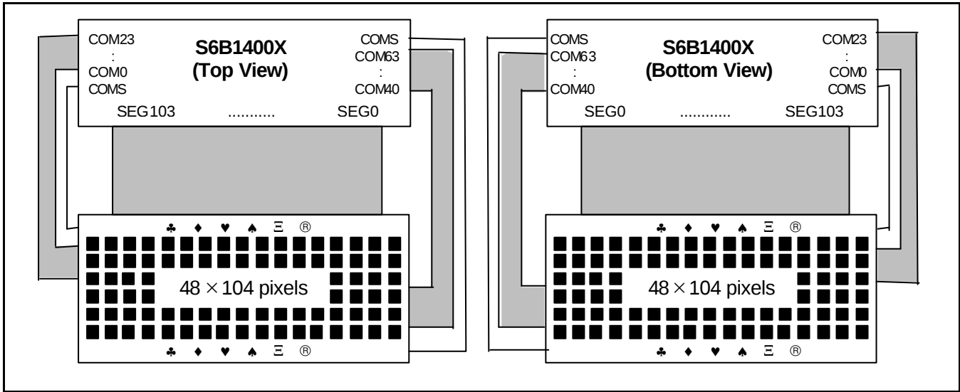
Figure 43. SHL = 0, ADC = 1
