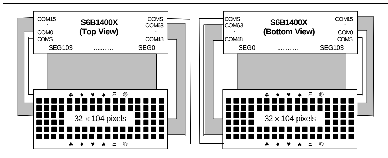
Figure 47. SHL = 0, ADC = 1
