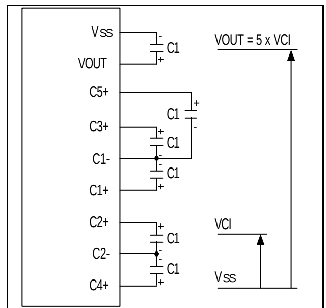
Figure 22. Six Times Boosting Circuit
