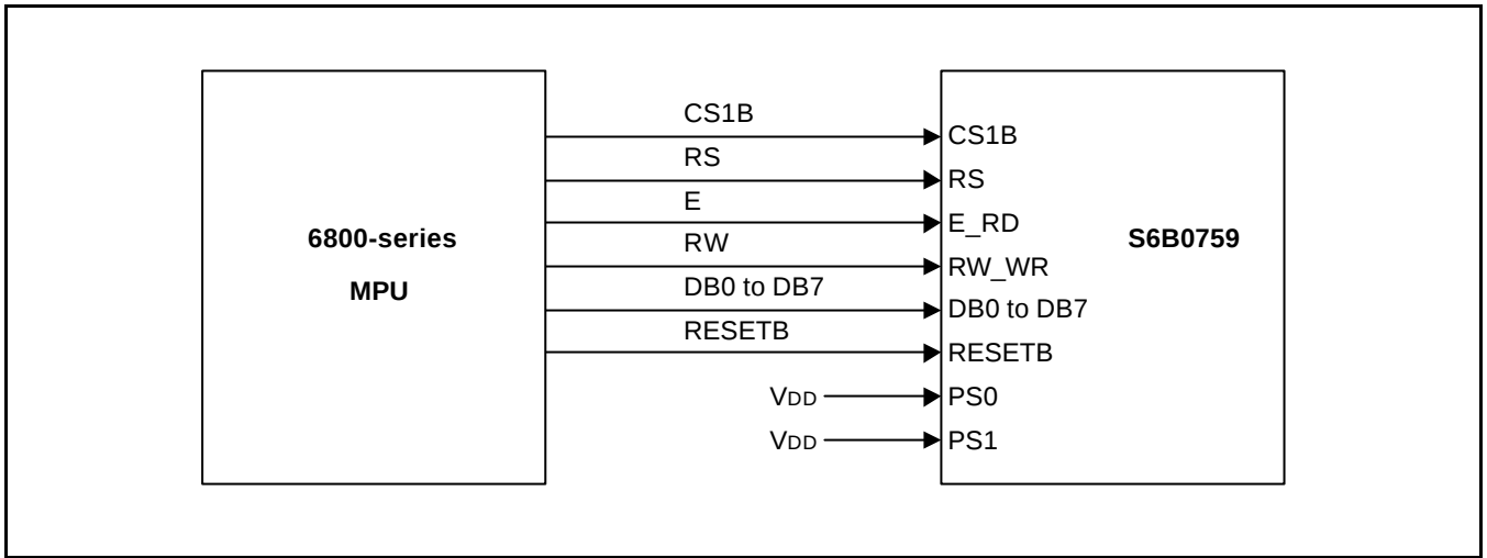
Figure 47. Interfacing with 6800-series
