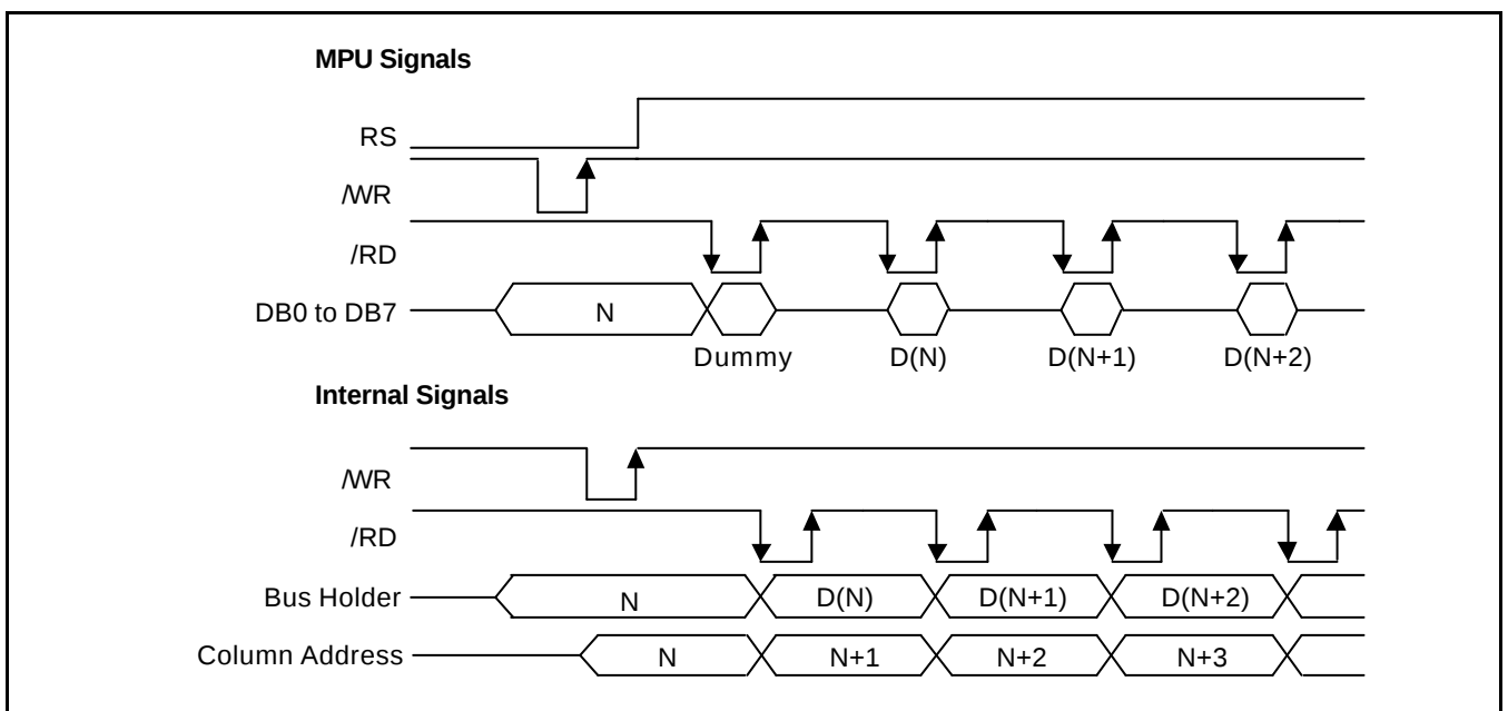
Figure 8. Read Timing
