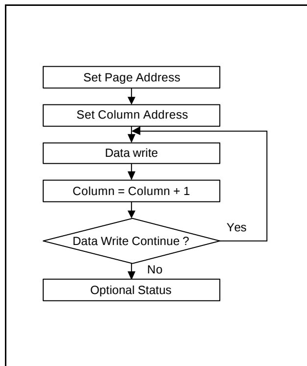
Figure 29. Sequence for Writing Display Data
