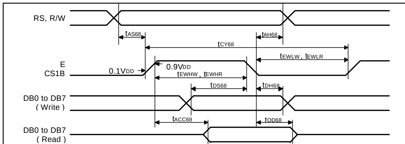
Figure 39. Parallel Interface (6800-series MPU) Timing Diagram
