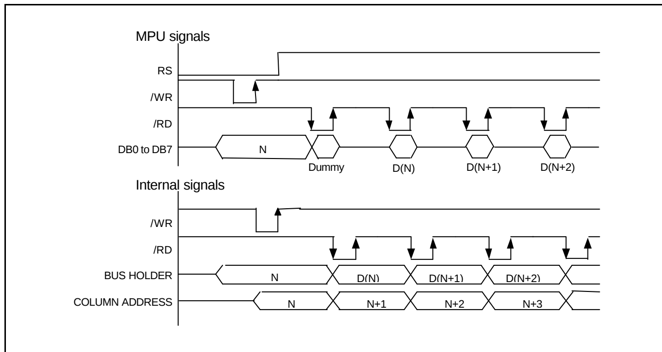
Figure 10. Read Timing
