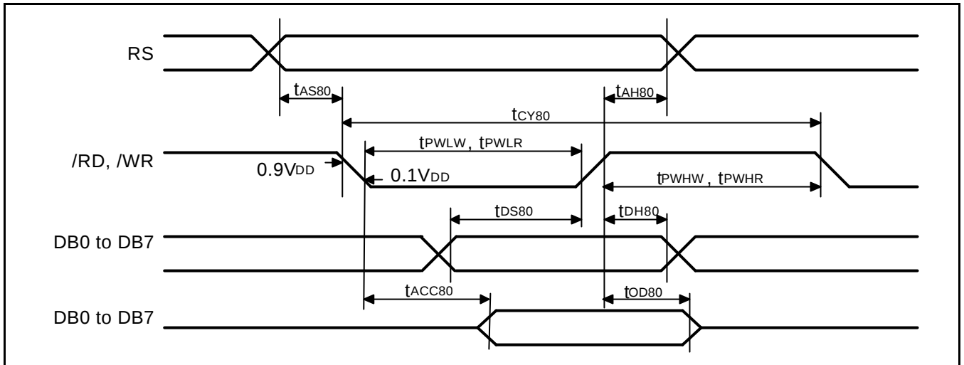
Figure 38. Parallel Interface (8080-series MPU) Timing Diagram
