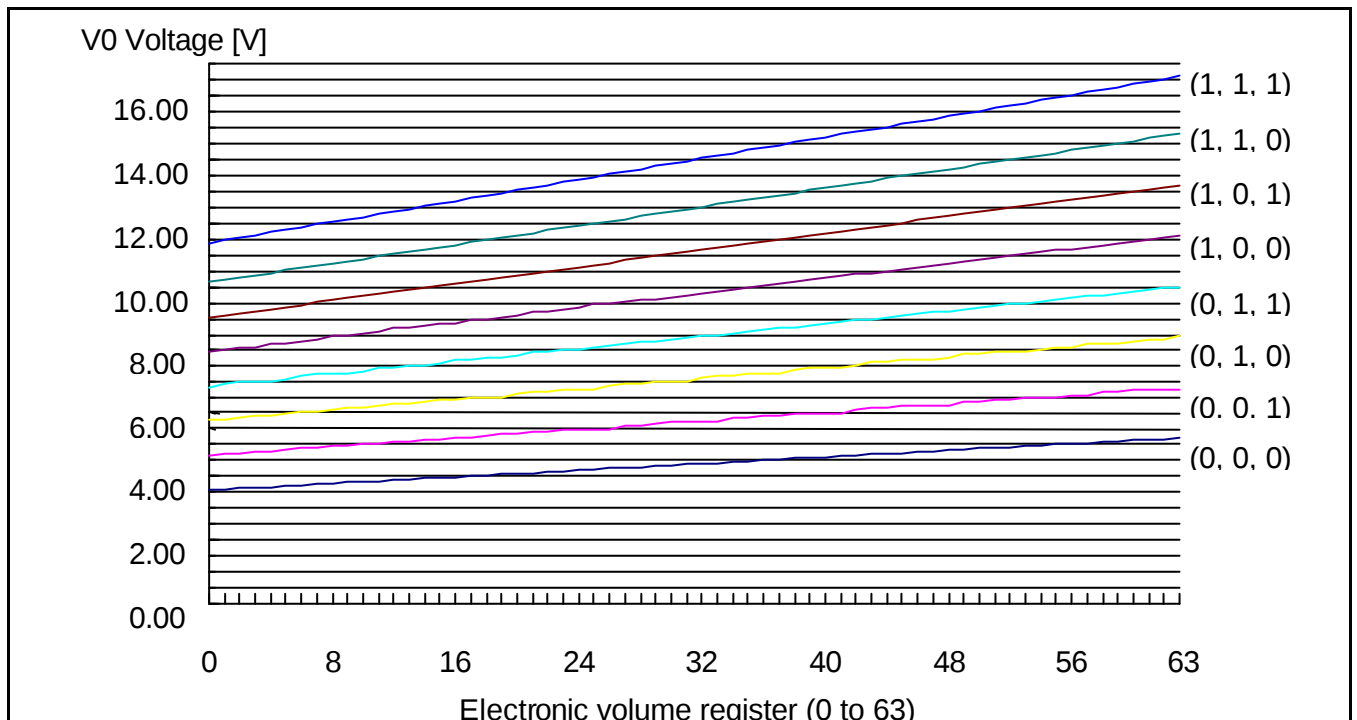
Figure 20. V0 Voltage by 1 + (R_b / R_a) and Electronic Volume Levels
