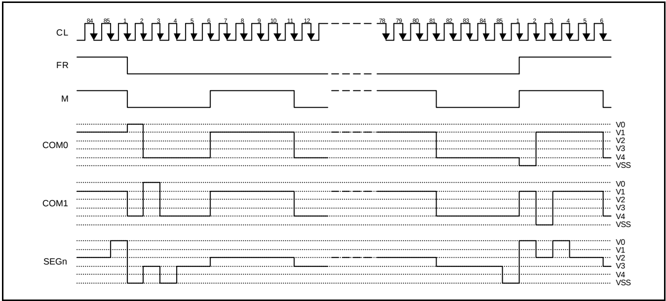
Figure 15. N-line Inversion Driving Waveform (N = 5, Duty Ratio = 1/85)
