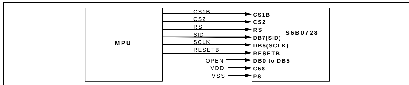
Figure 44. In Case of 4-Pin SPI Interface (PS = "L", C68 = "H")
