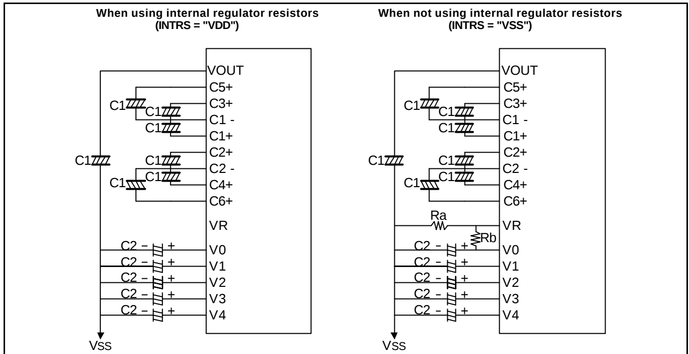
Figure 21. When Using all LCD Power Circuits (7-times V/C: ON, V/R: ON, V/F: ON)
