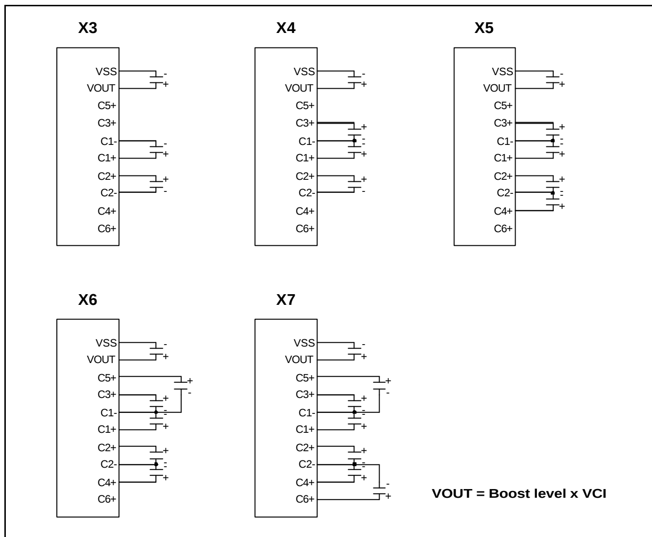
Figure 18. Boosting Circuits
