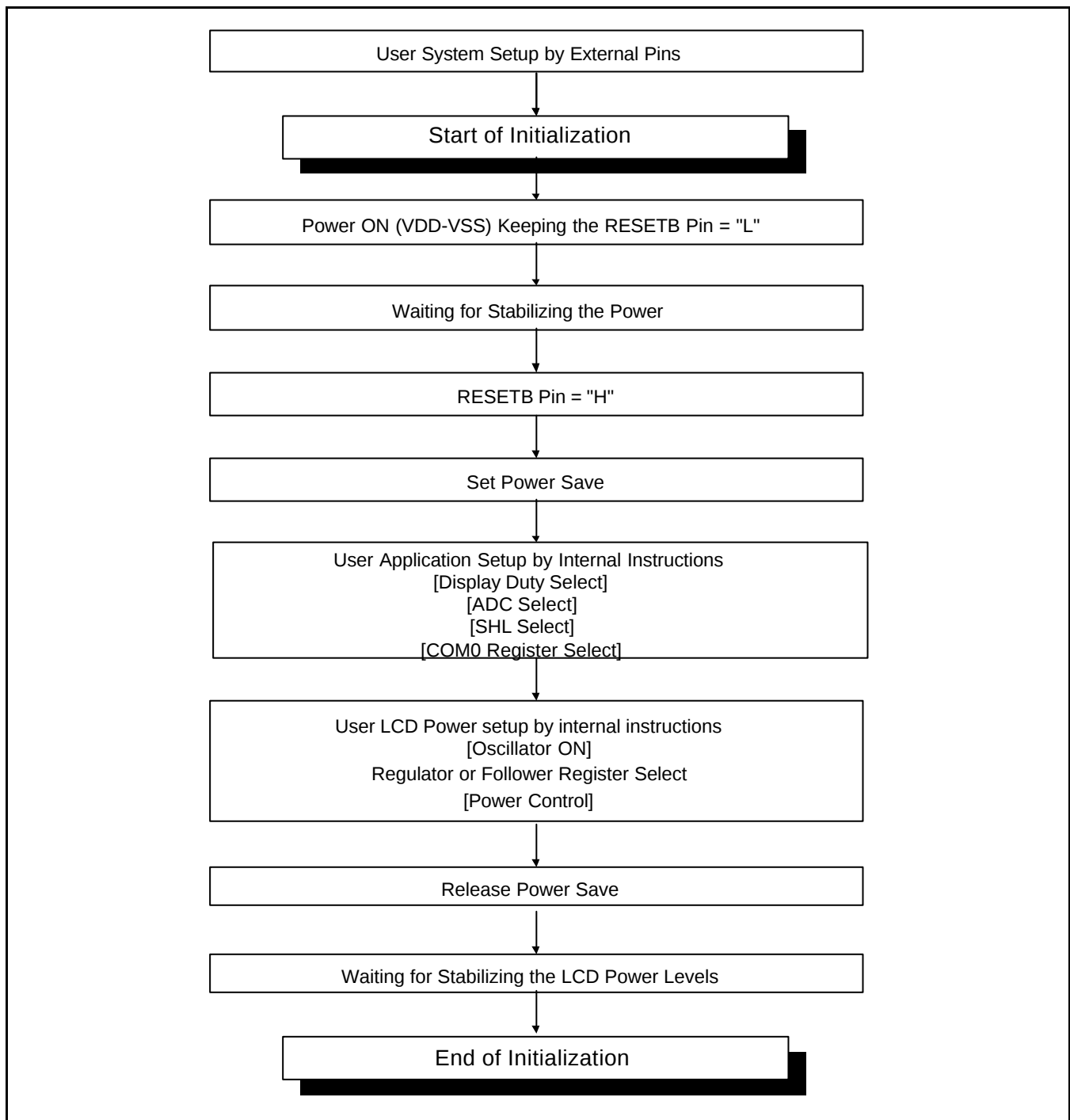
Figure 34. Initializing without the Built-in Power Supply Circuits
