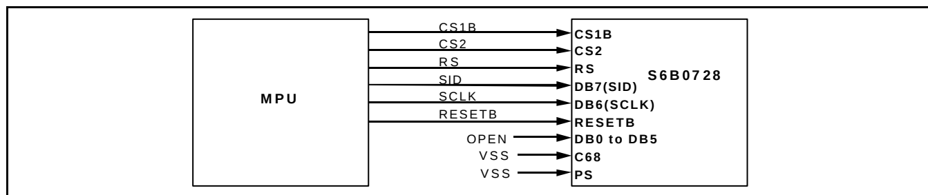
Figure 45. In Case of 3-Pin SPI Interface (PS = "L", C68 = "L")
