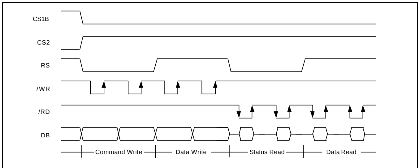
Figure 6. 8080-Series MPU Interface Protocol (PS="H", C68="L")
