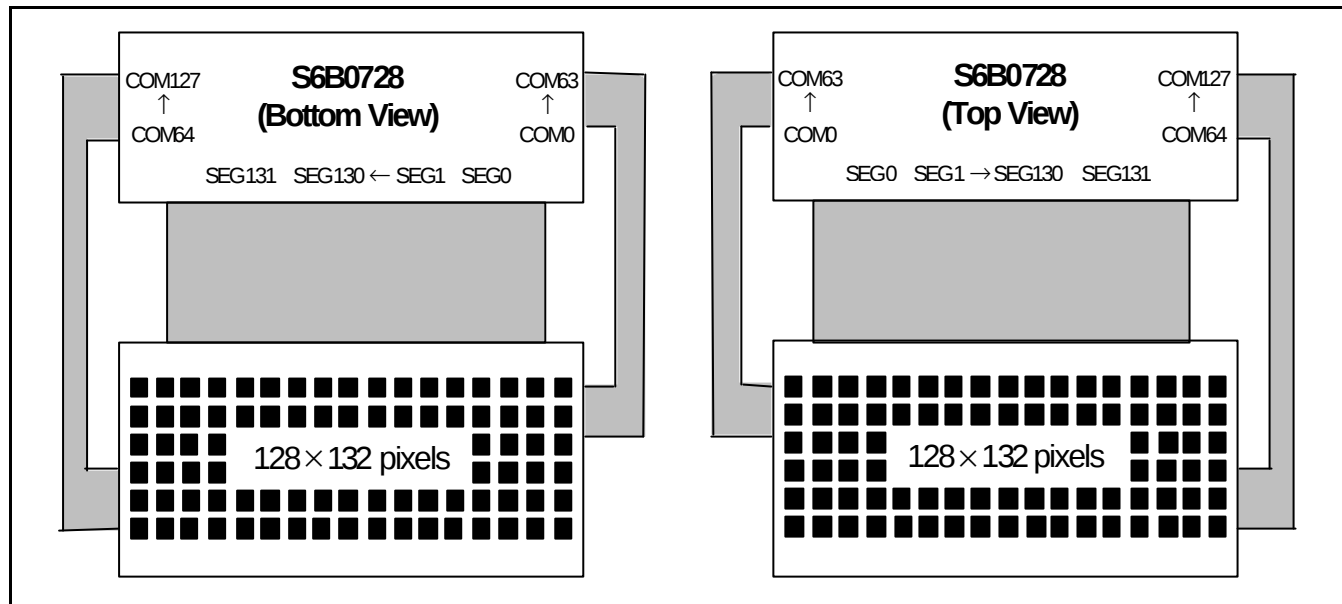
Figure 46. SHL = 0, ADC = 0
