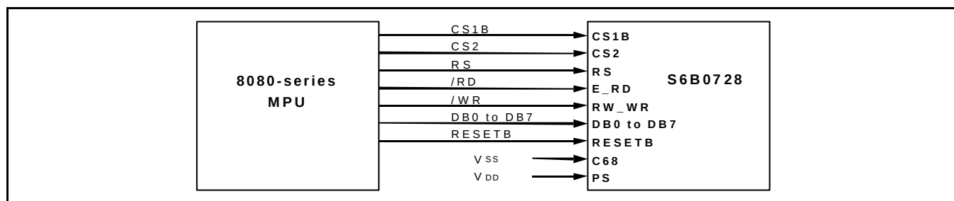
Figure 43. In Case of Interfacing with 8080-series (PS = "H", C68 = "L")
