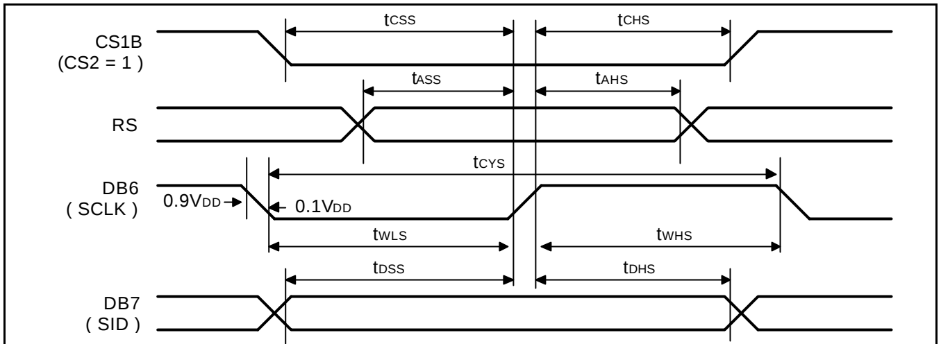
Figure 40. Serial Interface Timing Diagram
