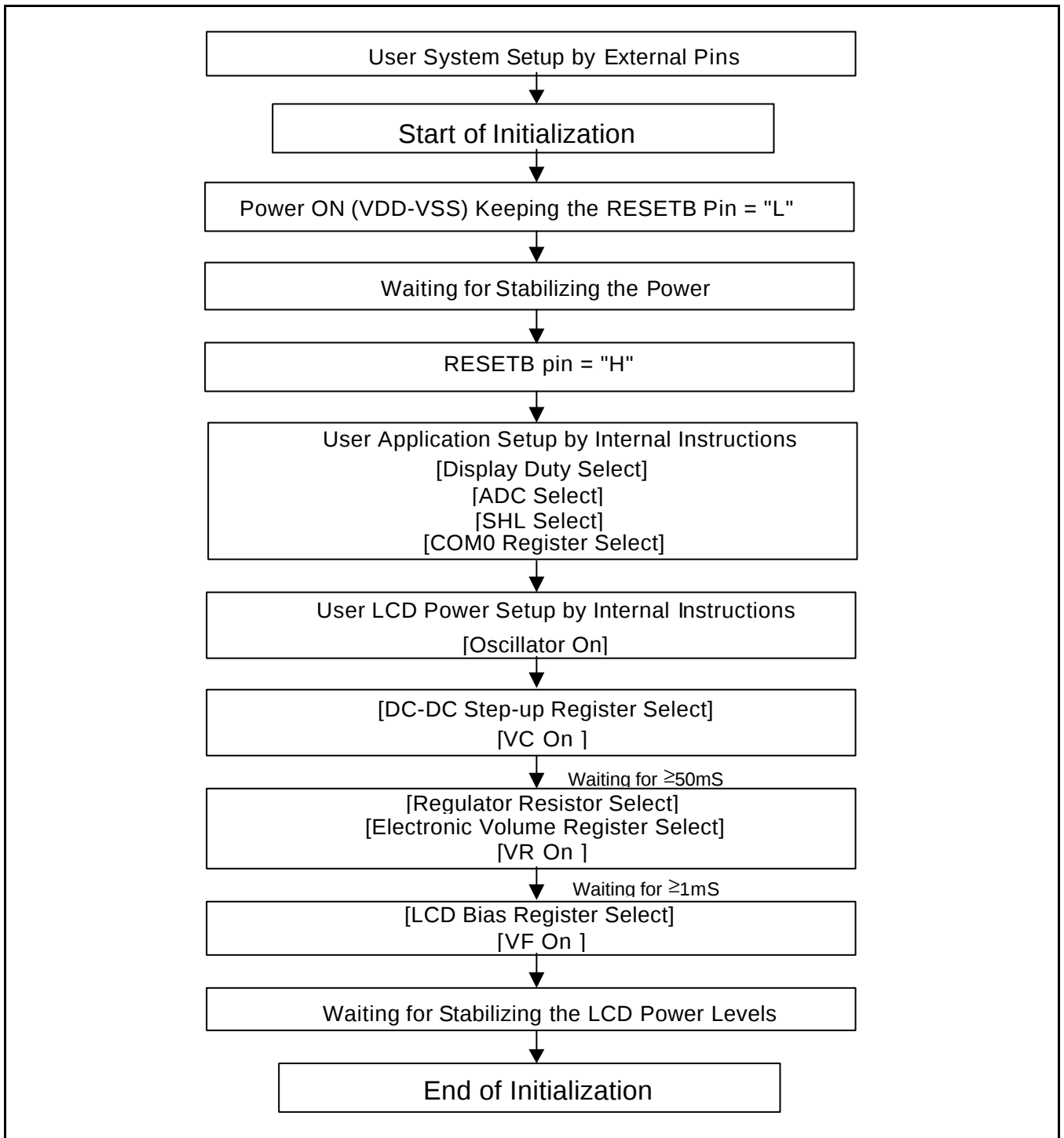
Figure 33. Initializing with the Built-in Power Supply Circuits
