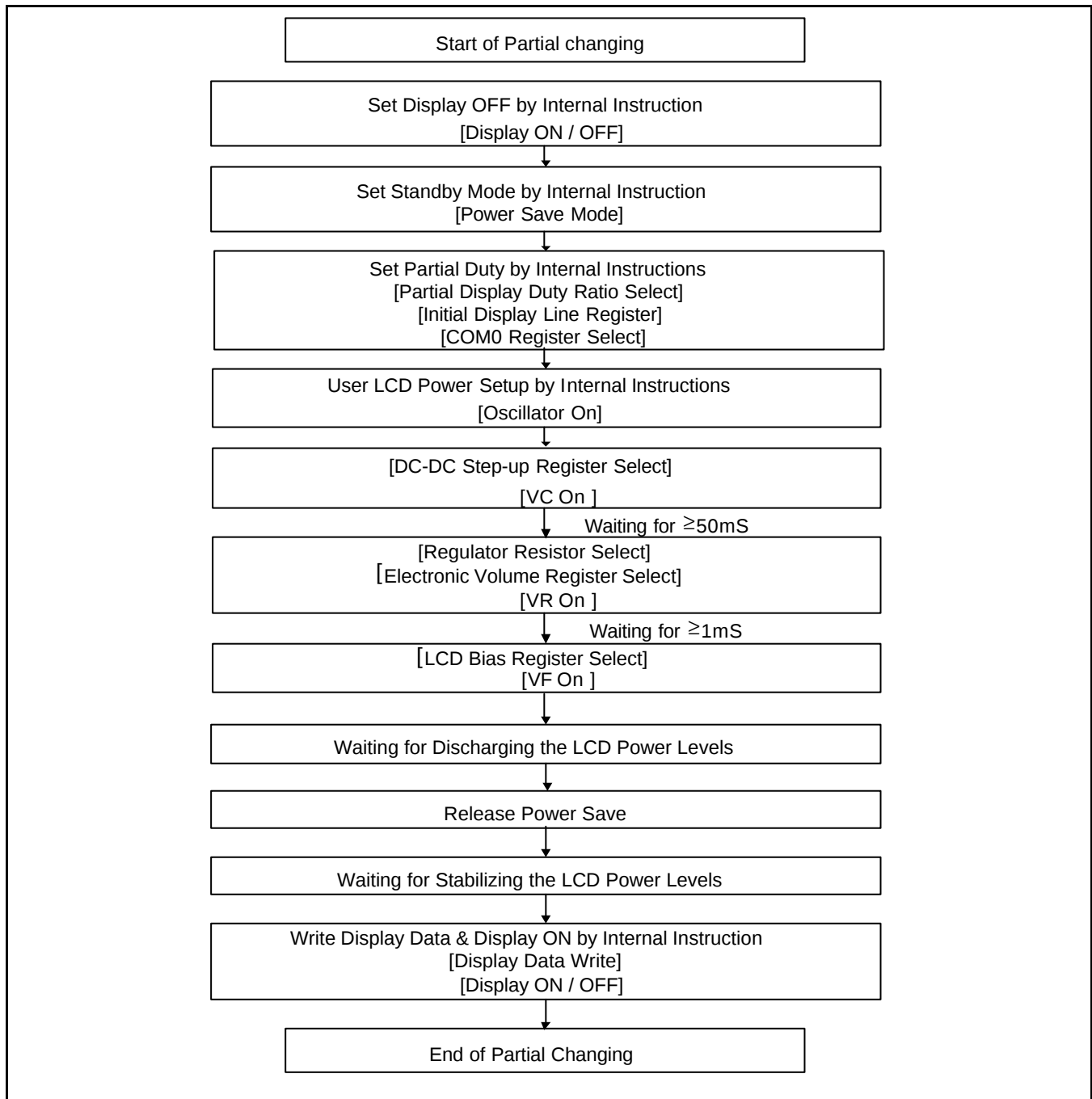
Figure 37. Partial Duty Changing
