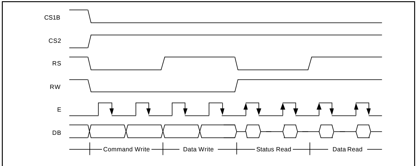
Figure 5. 6800-Series MPU Interface protocol (PS="H", C68="H")
