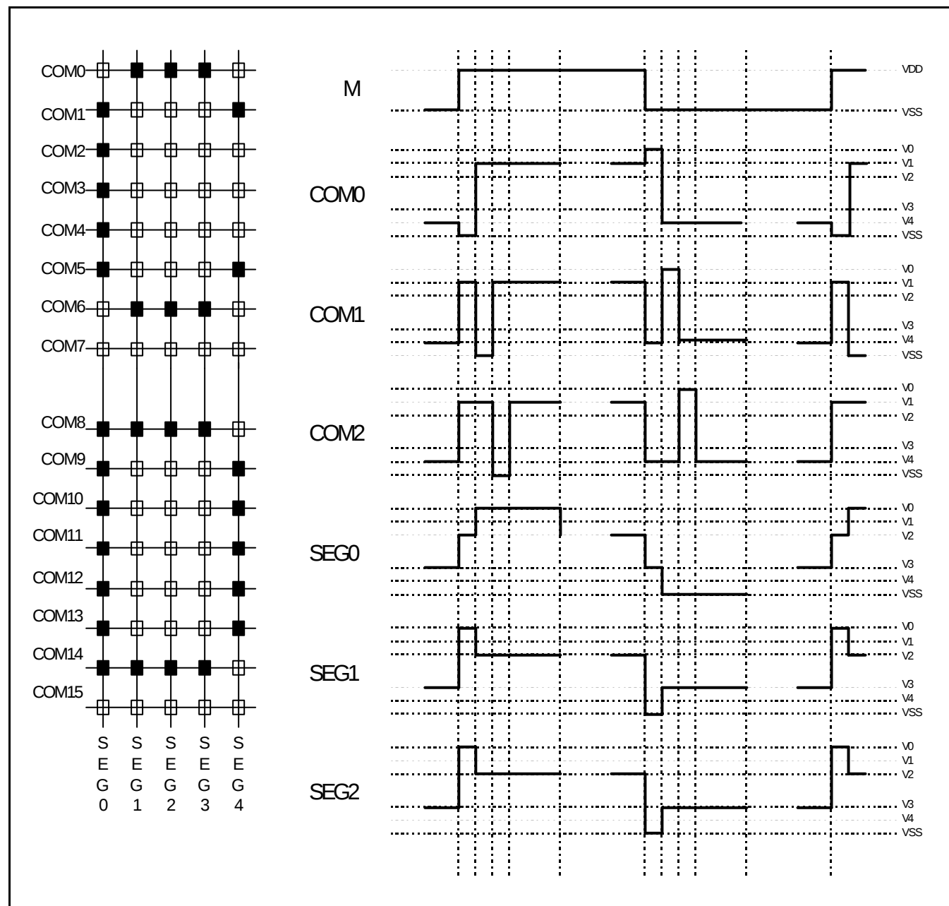
Figure 16. Segment and Common Timing
