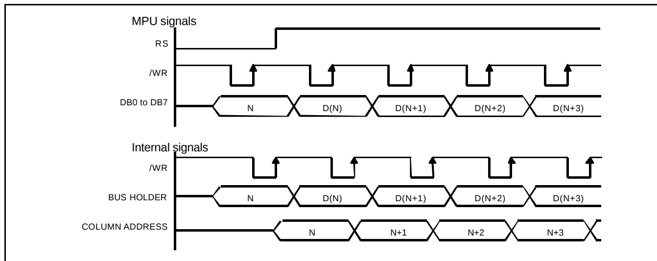
Figure 9. Write Timing
