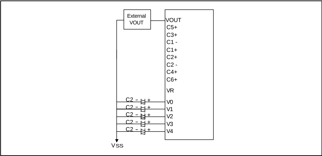
Figure 23. When Using only Voltage Follower Circuit (V/C: OFF, V/R: OFF, V/F: ON)
