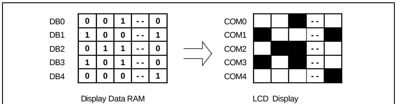
Figure 11. RAM-to-LCD Data Transfer
