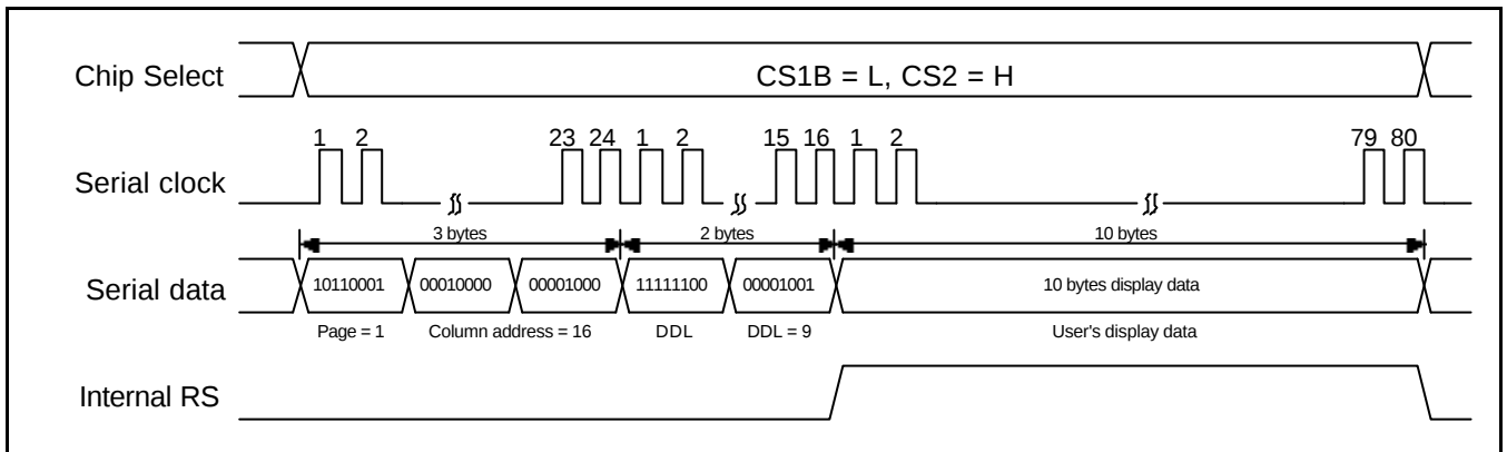
Figure 8. 3 Pin SPI Timing (RS is not used)
