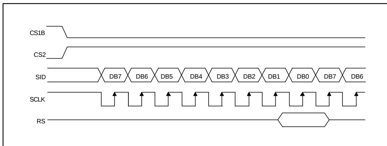
Figure 7. 4-Pin SPI Timing (RS is used)
