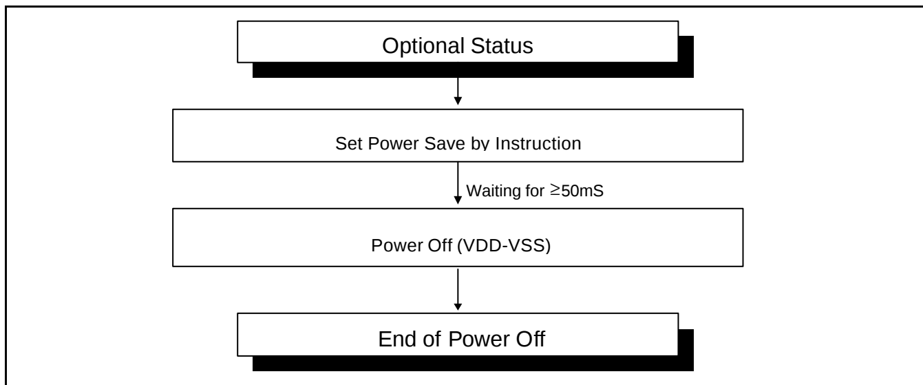
Figure 36. Power OFF
