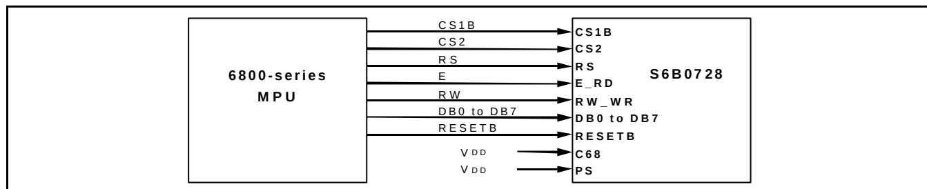
Figure 42. In Case of Interfacing with 6800-series (PS = "H", C68 = "H")
