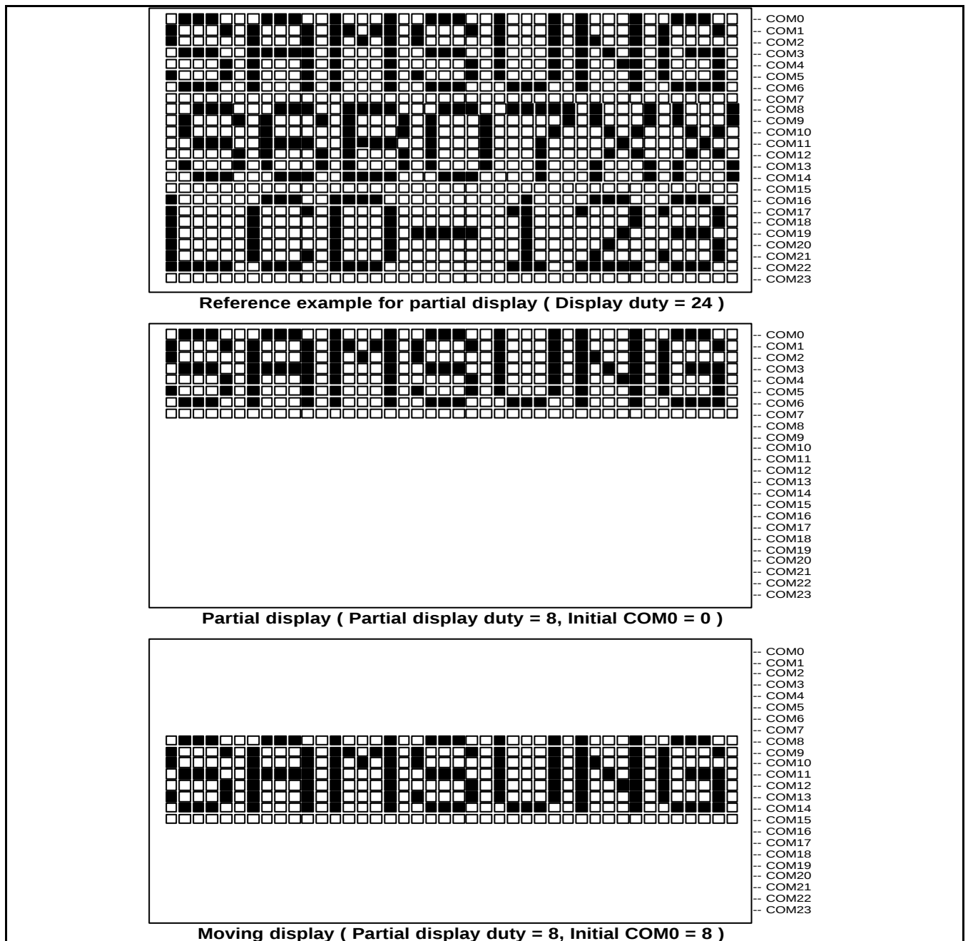
Figure 17. Reference Example for Partial Display
