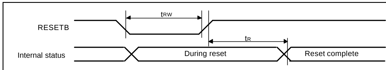
Figure 41. Reset Input Timing Diagram
