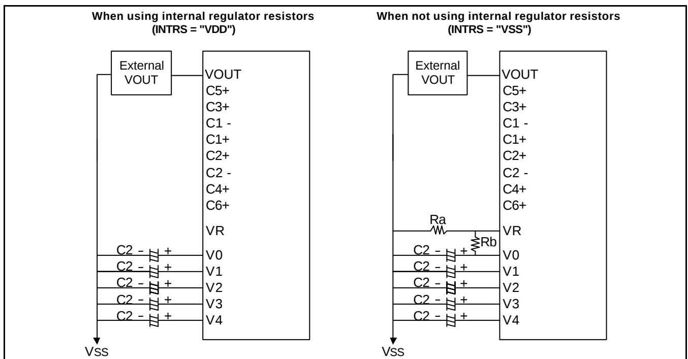
Figure 22. When Using some LCD Power Circuits (V/C: OFF, V/R: ON, V/F: ON)
