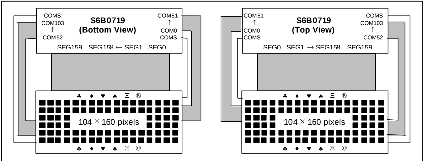
Figure 48. SHL = 0, ADC = 0 Figure 49. SHL = 0, ADC = 1
