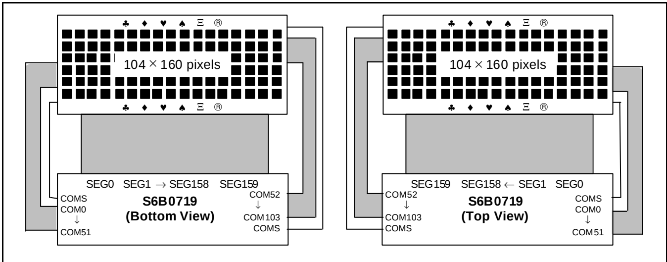
Figure 50. SHL = 1, ADC = 0 Figure 51. SHL = 1, ADC = 1
