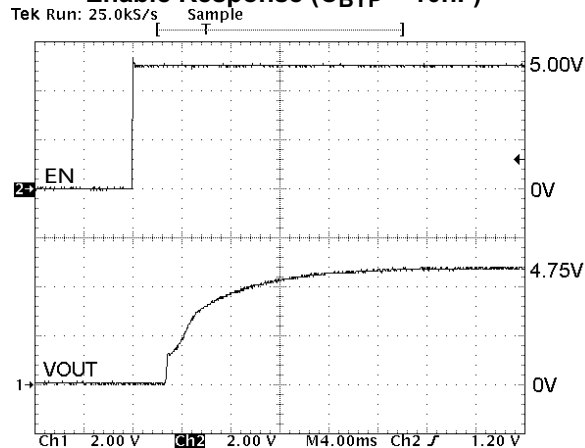
Enable Response ( C_{BYP} = 10nF )
