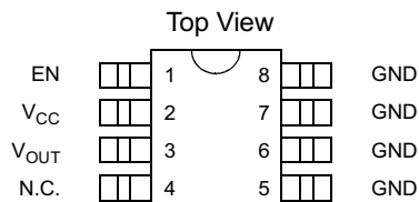
8-pin SOIC
