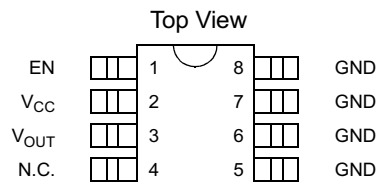
8-pin MSOP (CM3002-33MA only)
