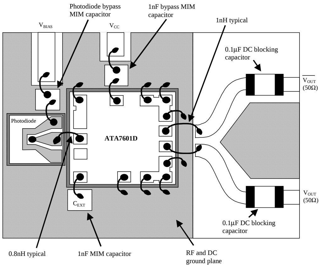
Figure 8: Bonding Diagram
