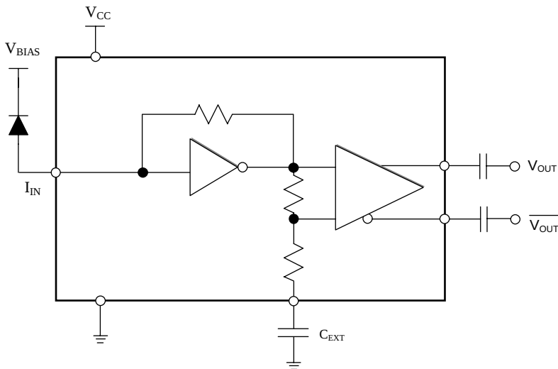
Figure 1: Circuit Block Diagram
