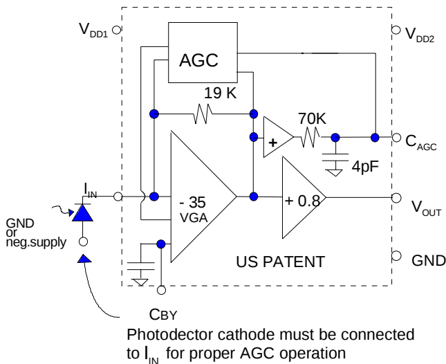
Figure 1: Equivalent Circuit
