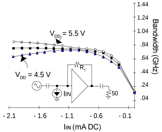
Figure 9: Bandwidth vs. I IN
