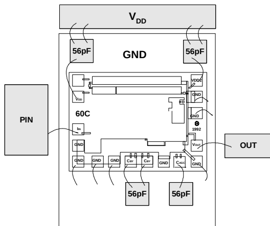
Figure 4: ATA 00501D1C Typical Bonding
