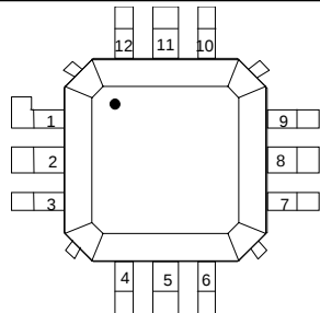
Figure 3: Pin Layout
