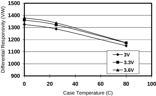
Figure 8: Differential Responsivity vs. Temperature
