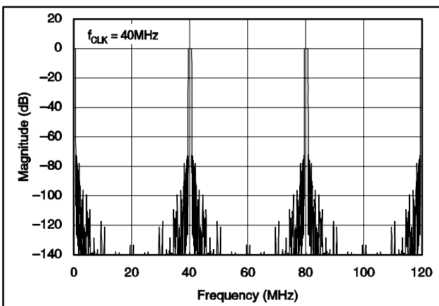
Figure 22. Frequency Response Out to 120MHz
