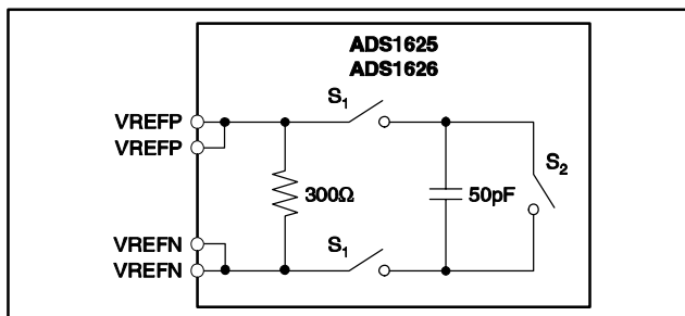
Figure 13. Conceptual Internal Circuitry for the Reference When \overline{REFEN} = \text{High}
