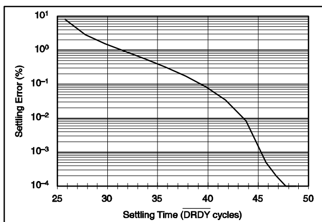
Figure 17. Settling Time
