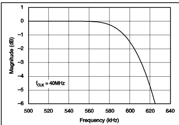
Figure 21. Passband Transition
