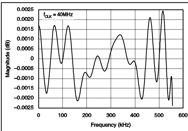
Figure 20. Passband Ripple
