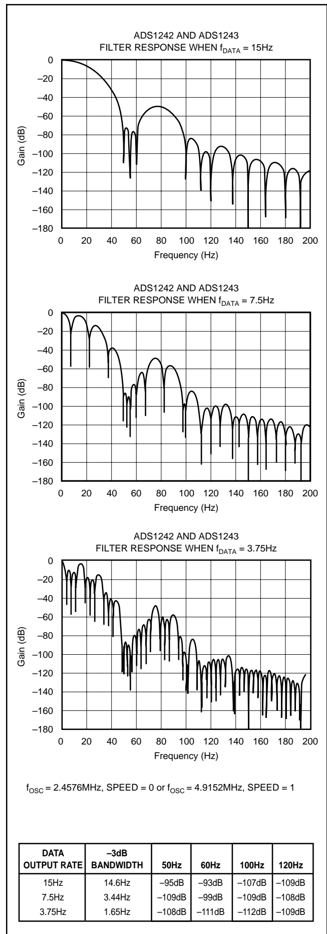
FIGURE 2. Filter Frequency Responses.
