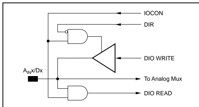
FIGURE 4. Analog/Data Interface Pin.
